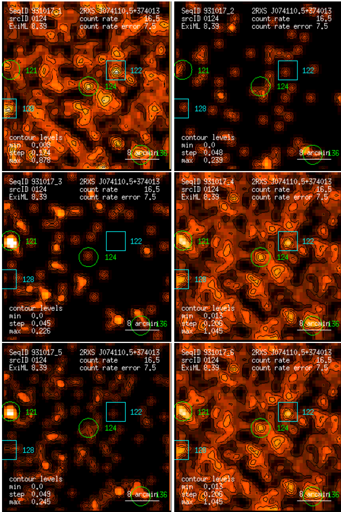
Figure 124: RASS 931017: detection 0124: band rate images, Gaussian filter: (1) PSPC channels 11 – 41, (2) 52 – 90, (3) 91 – 201, (4) 11 – 235, (5) 52 – 201, (6) 11 – 201. Broad band rates in counts/ks. Band rate contour levels in counts/ks/arcmin 2 .
