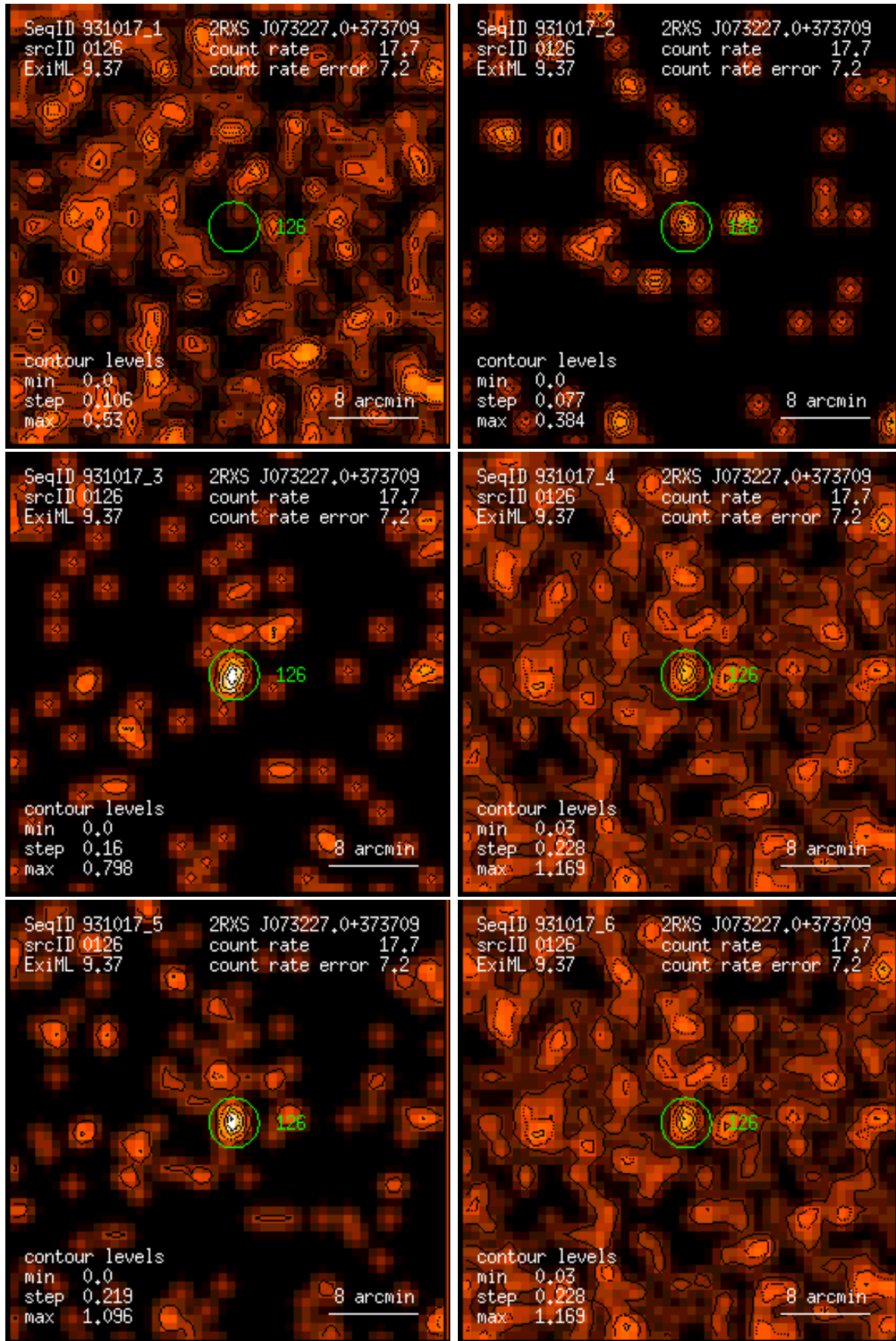
Figure 126: RASS 931017: detection 0126: band rate images, Gaussian filter: (1) PSPC channels 11 – 41, (2) 52 – 90, (3) 91 – 201, (4) 11 – 235, (5) 52 – 201, (6) 11 – 201. Broad band rates in counts/ks. Band rate contour levels in counts/ks/arcmin 2 .
