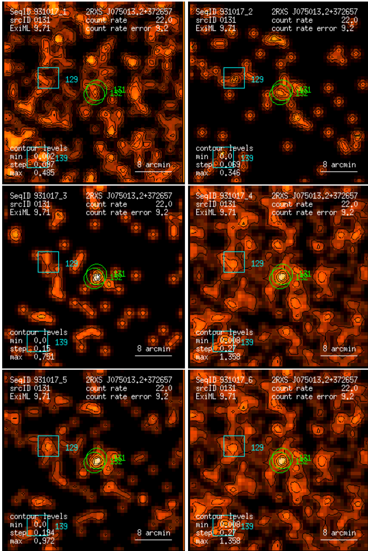
Figure 131: RASS 931017: detection 0131: band rate images, Gaussian filter: (1) PSPC channels 11 – 41, (2) 52 – 90, (3) 91 – 201, (4) 11 – 235, (5) 52 – 201, (6) 11 – 201. Broad band rates in counts/ks. Band rate contour levels in counts/ks/arcmin 2 .
