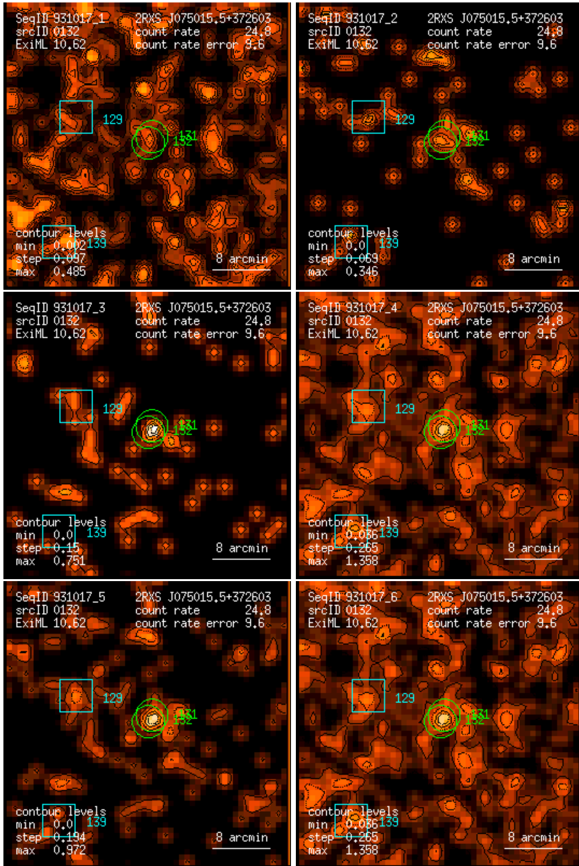
Figure 132: RASS 931017: detection 0132: band rate images, Gaussian filter: (1) PSPC channels 11 – 41, (2) 52 – 90, (3) 91 – 201, (4) 11 – 235, (5) 52 – 201, (6) 11 – 201. Broad band rates in counts/ks. Band rate contour levels in counts/ks/arcmin 2 .
