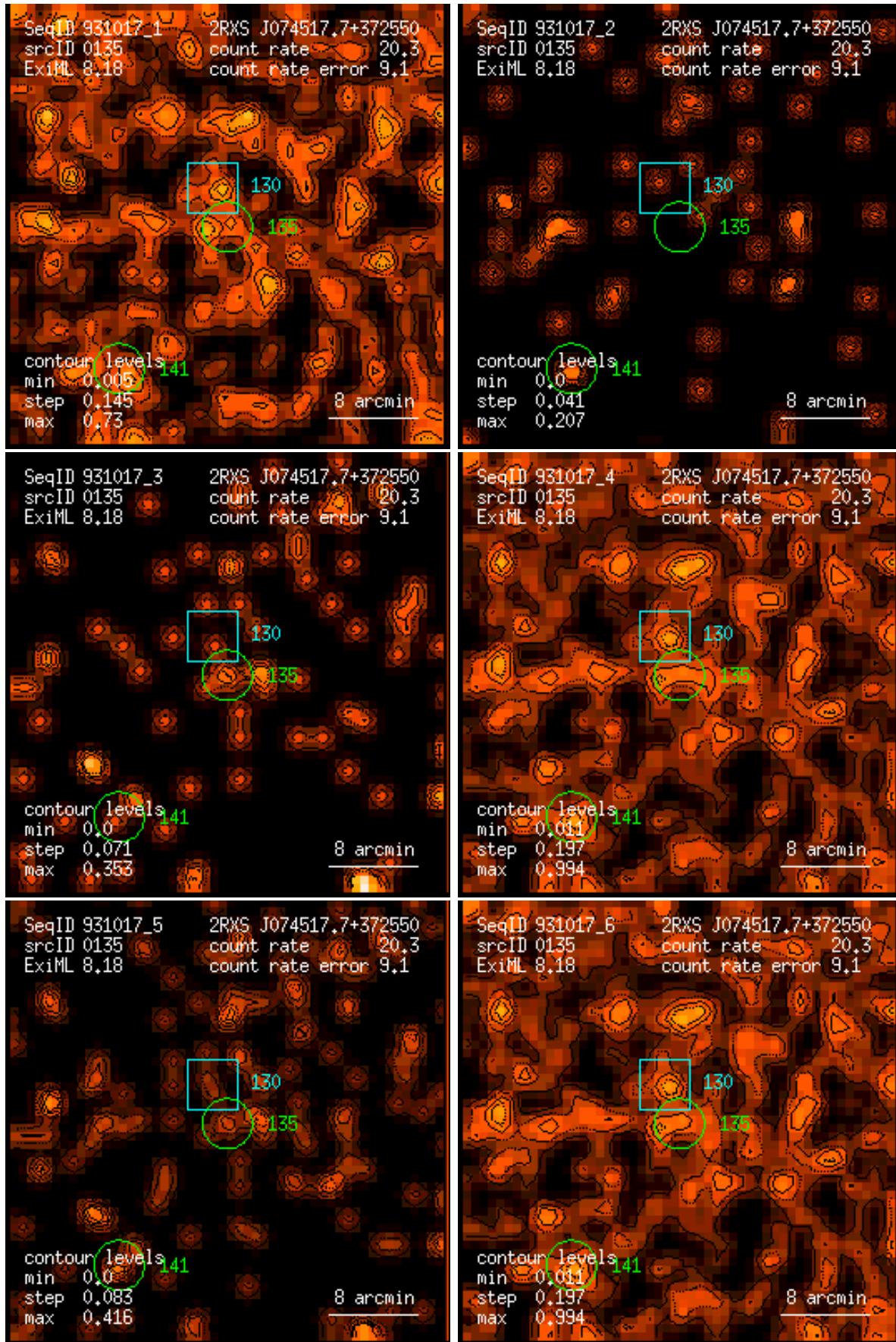
Figure 135: RASS 931017: detection 0135: band rate images, Gaussian filter: (1) PSPC channels 11 – 41, (2) 52 – 90, (3) 91 – 201, (4) 11 – 235, (5) 52 – 201, (6) 11 – 201. Broad band rates in counts/ks. Band rate contour levels in counts/ks/arcmin 2 .
