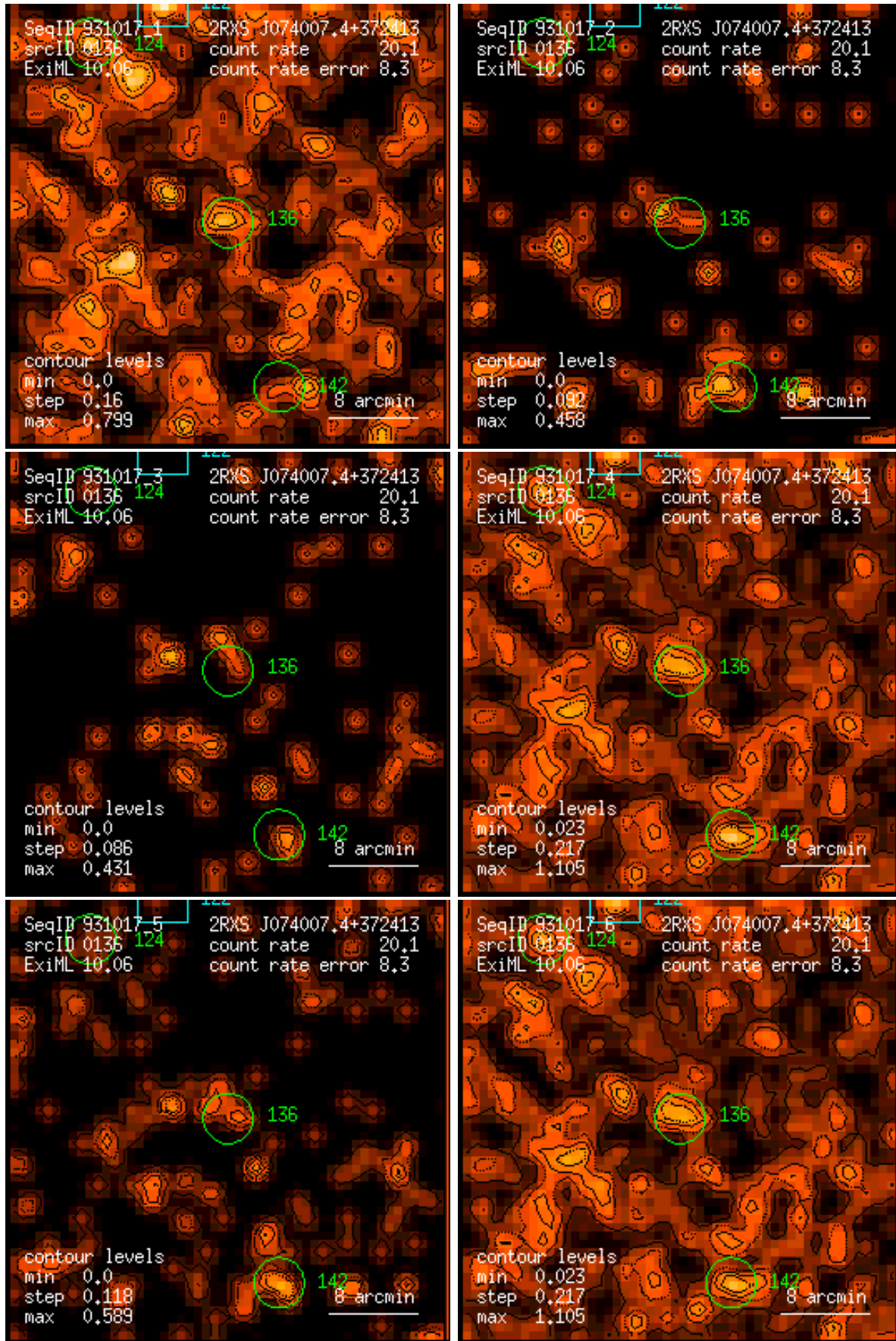
Figure 136: RASS 931017: detection 0136: band rate images, Gaussian filter: (1) PSPC channels 11 – 41, (2) 52 – 90, (3) 91 – 201, (4) 11 – 235, (5) 52 – 201, (6) 11 – 201. Broad band rates in counts/ks. Band rate contour levels in counts/ks/arcmin 2 .
