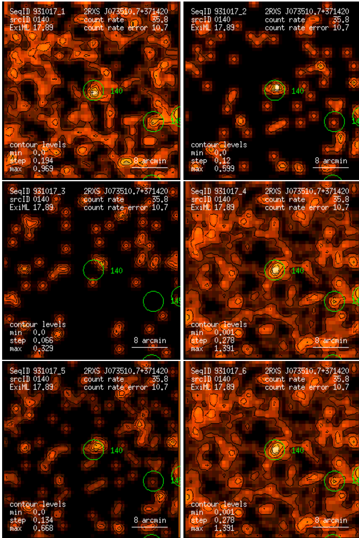
Figure 140: RASS 931017: detection 0140: band rate images, Gaussian filter: (1) PSPC channels 11 – 41, (2) 52 – 90, (3) 91 – 201, (4) 11 – 235, (5) 52 – 201, (6) 11 – 201. Broad band rates in counts/ks. Band rate contour levels in counts/ks/arcmin 2 .
