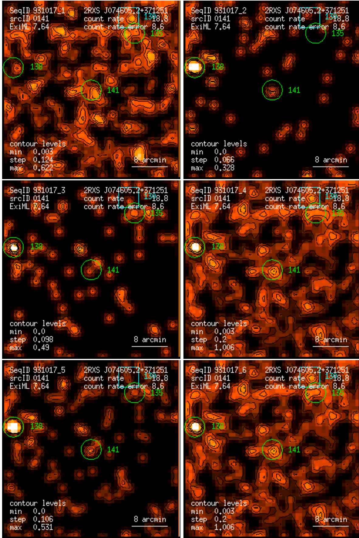
Figure 141: RASS 931017: detection 0141: band rate images, Gaussian filter: (1) PSPC channels 11 – 41, (2) 52 – 90, (3) 91 – 201, (4) 11 – 235, (5) 52 – 201, (6) 11 – 201. Broad band rates in counts/ks. Band rate contour levels in counts/ks/arcmin 2 .
