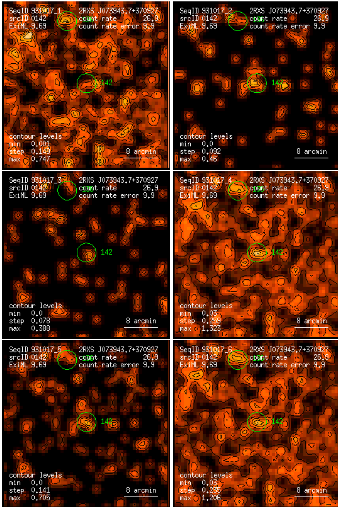
Figure 142: RASS 931017: detection 0142: band rate images, Gaussian filter: (1) PSPC channels 11 – 41, (2) 52 – 90, (3) 91 – 201, (4) 11 – 235, (5) 52 – 201, (6) 11 – 201. Broad band rates in counts/ks. Band rate contour levels in counts/ks/arcmin 2 .
