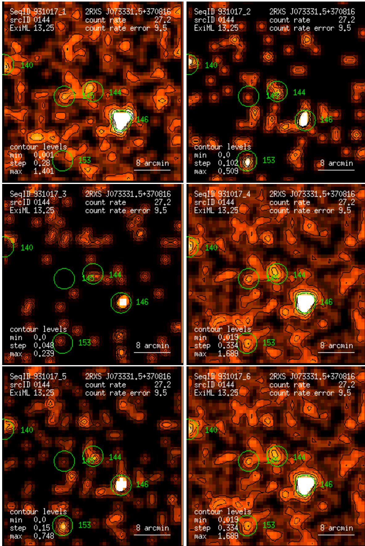
Figure 144: RASS 931017: detection 0144: band rate images, Gaussian filter: (1) PSPC channels 11 – 41, (2) 52 – 90, (3) 91 – 201, (4) 11 – 235, (5) 52 – 201, (6) 11 – 201. Broad band rates in counts/ks. Band rate contour levels in counts/ks/arcmin 2 .
