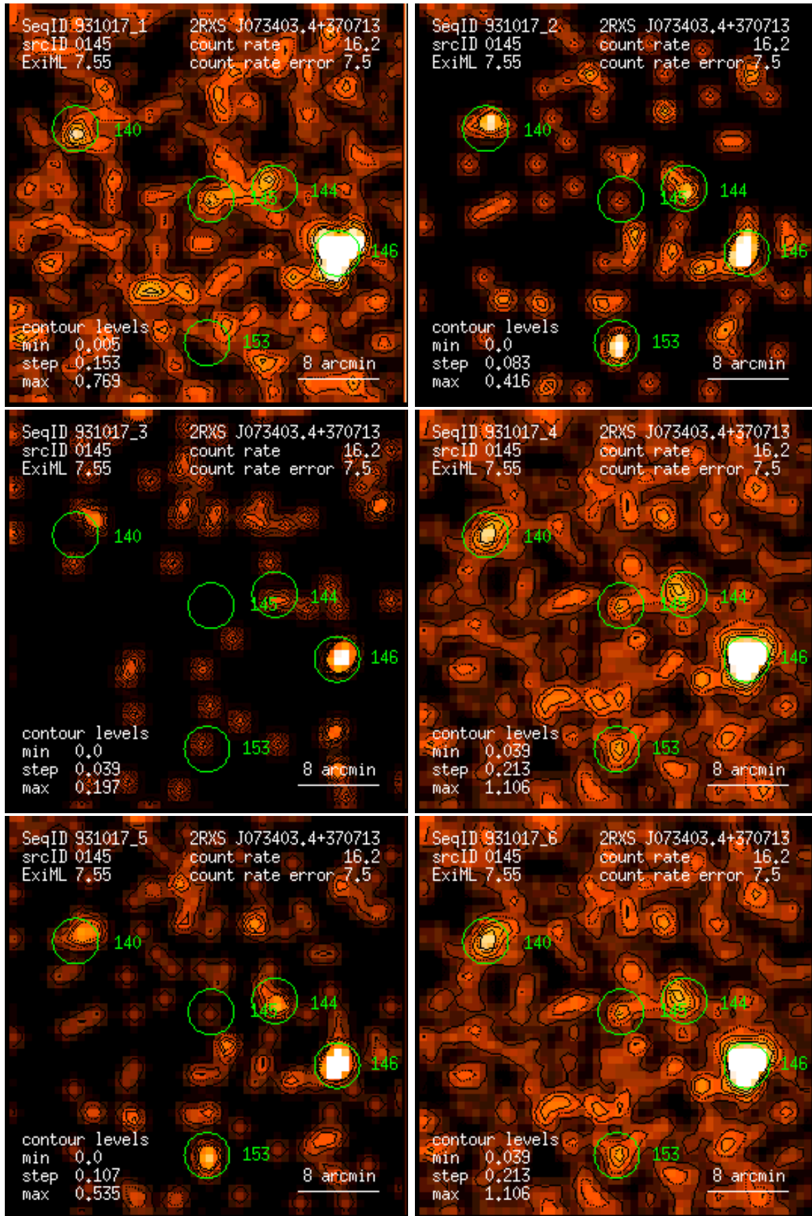
Figure 145: RASS 931017: detection 0145: band rate images, Gaussian filter: (1) PSPC channels 11 – 41, (2) 52 – 90, (3) 91 – 201, (4) 11 – 235, (5) 52 – 201, (6) 11 – 201. Broad band rates in counts/ks. Band rate contour levels in counts/ks/arcmin 2 .
