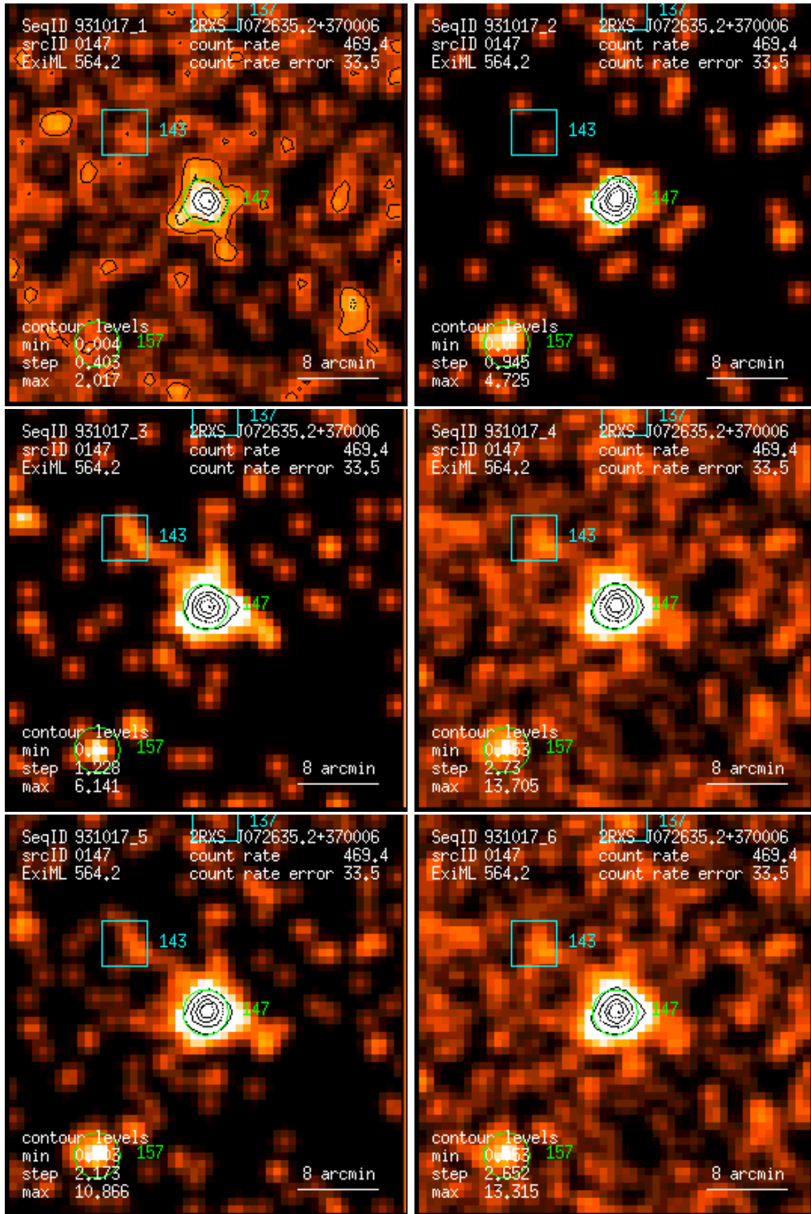
Figure 147: RASS 931017: detection 0147: band rate images, Gaussian filter: (1) PSPC channels 11 – 41, (2) 52 – 90, (3) 91 – 201, (4) 11 – 235, (5) 52 – 201, (6) 11 – 201. Broad band rates in counts/ks. Band rate contour levels in counts/ks/arcmin 2 .
