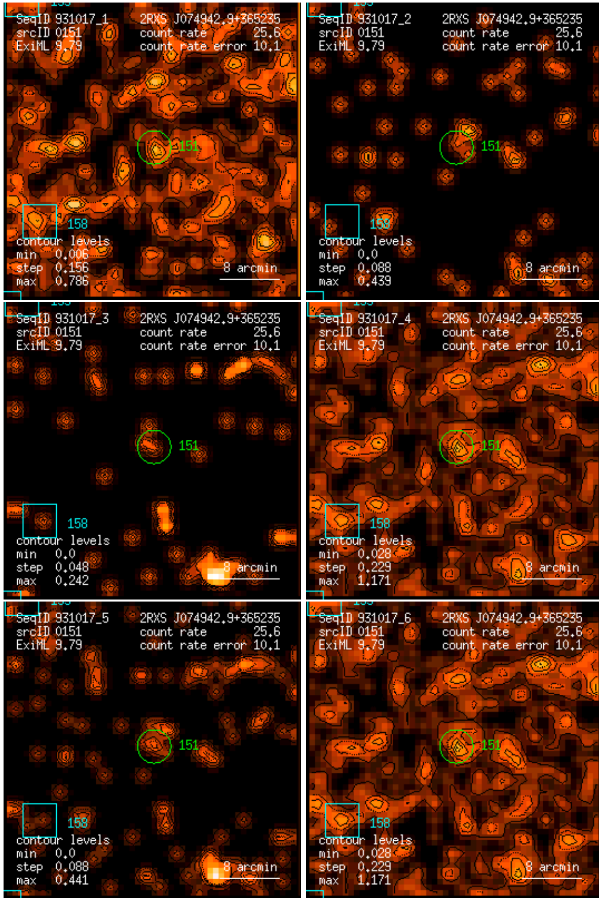
Figure 151: RASS 931017: detection 0151: band rate images, Gaussian filter: (1) PSPC channels 11 – 41, (2) 52 – 90, (3) 91 – 201, (4) 11 – 235, (5) 52 – 201, (6) 11 – 201. Broad band rates in counts/ks. Band rate contour levels in counts/ks/arcmin 2 .
