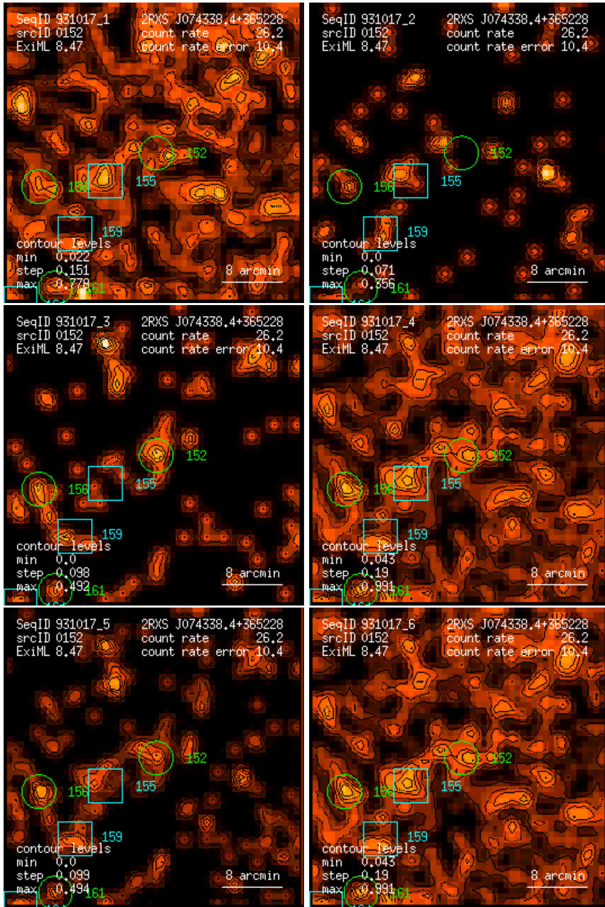
Figure 152: RASS 931017: detection 0152: band rate images, Gaussian filter: (1) PSPC channels 11 – 41, (2) 52 – 90, (3) 91 – 201, (4) 11 – 235, (5) 52 – 201, (6) 11 – 201. Broad band rates in counts/ks. Band rate contour levels in counts/ks/arcmin 2 .
