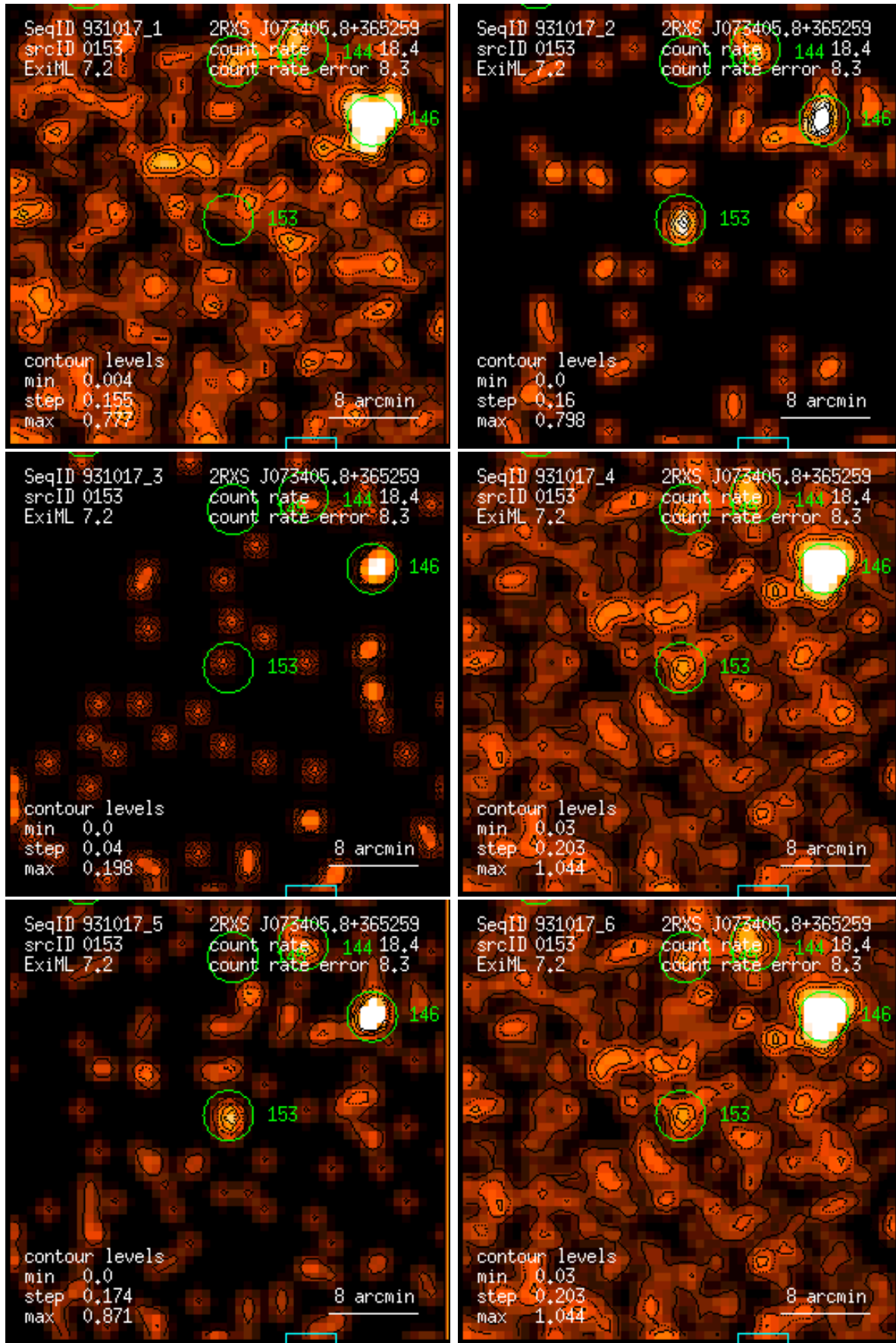
Figure 153: RASS 931017: detection 0153: band rate images, Gaussian filter: (1) PSPC channels 11 – 41, (2) 52 – 90, (3) 91 – 201, (4) 11 – 235, (5) 52 – 201, (6) 11 – 201. Broad band rates in counts/ks. Band rate contour levels in counts/ks/arcmin 2 .
