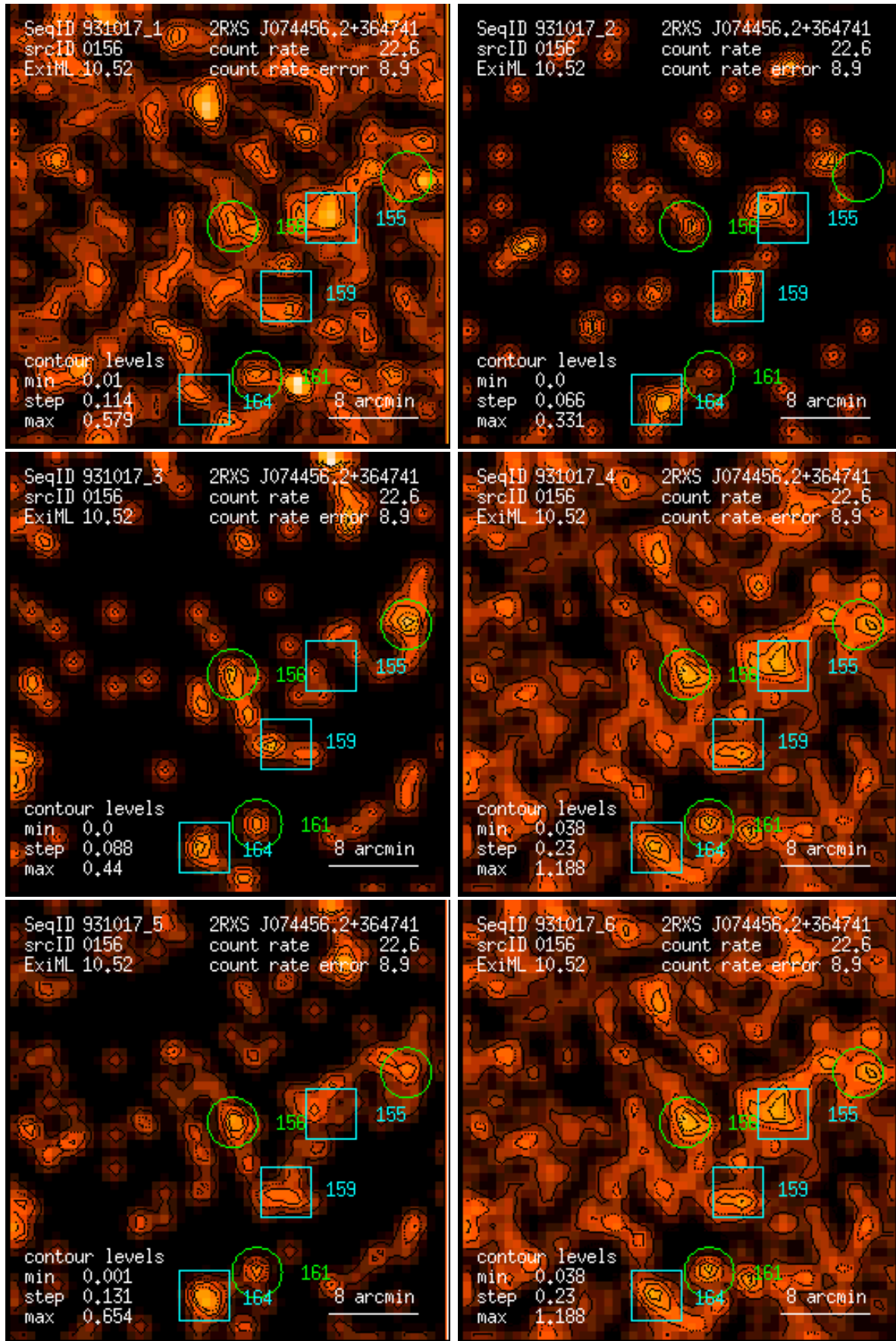
Figure 156: RASS 931017: detection 0156: band rate images, Gaussian filter: (1) PSPC channels 11 – 41, (2) 52 – 90, (3) 91 – 201, (4) 11 – 235, (5) 52 – 201, (6) 11 – 201. Broad band rates in counts/ks. Band rate contour levels in counts/ks/arcmin 2 .
