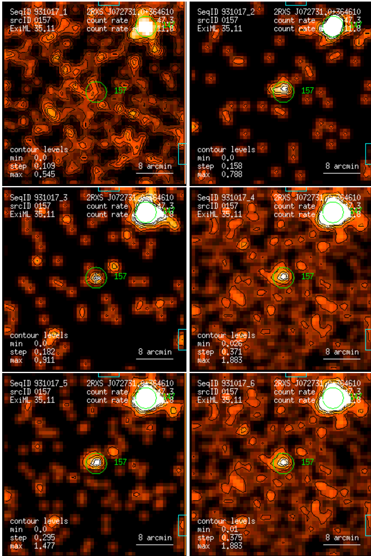
Figure 157: RASS 931017: detection 0157: band rate images, Gaussian filter: (1) PSPC channels 11 – 41, (2) 52 – 90, (3) 91 – 201, (4) 11 – 235, (5) 52 – 201, (6) 11 – 201. Broad band rates in counts/ks. Band rate contour levels in counts/ks/arcmin 2 .
