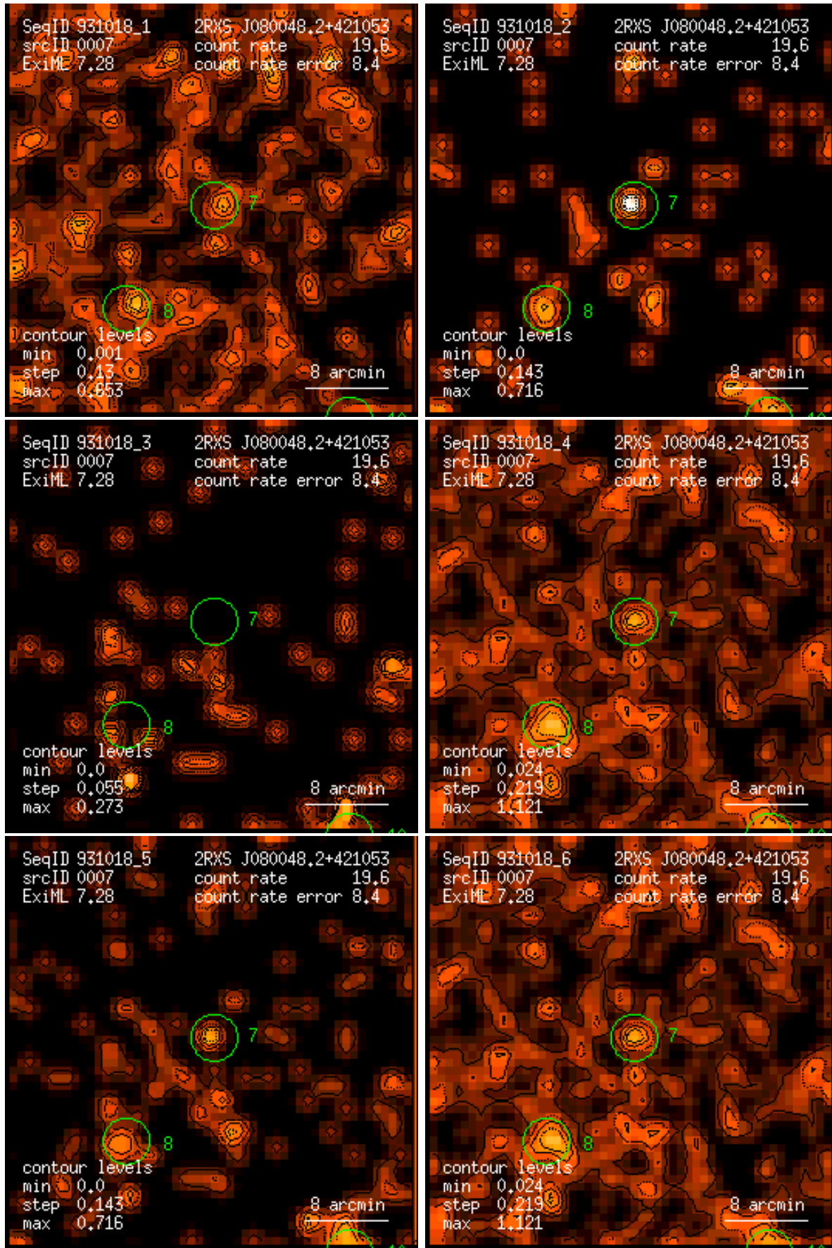
Figure 7: RASS 931018: detection 0007: band rate images, Gaussian filter: (1) PSPC channels 11 – 41, (2) 52 – 90, (3) 91 – 201, (4) 11 – 235, (5) 52 – 201, (6) 11 – 201. Broad band rates in counts/ks. Band rate contour levels in counts/ks/arcmin 2 .
