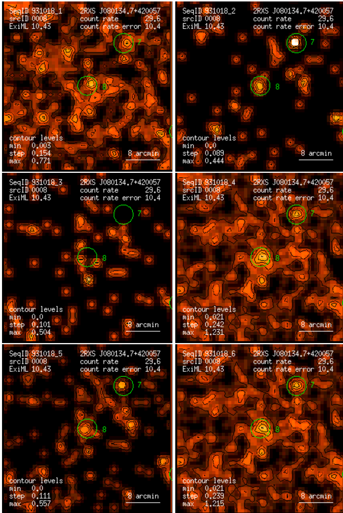
Figure 8: RASS 931018: detection 0008: band rate images, Gaussian filter: (1) PSPC channels 11 – 41, (2) 52 – 90, (3) 91 – 201, (4) 11 – 235, (5) 52 – 201, (6) 11 – 201. Broad band rates in counts/ks. Band rate contour levels in counts/ks/arcmin 2 .
