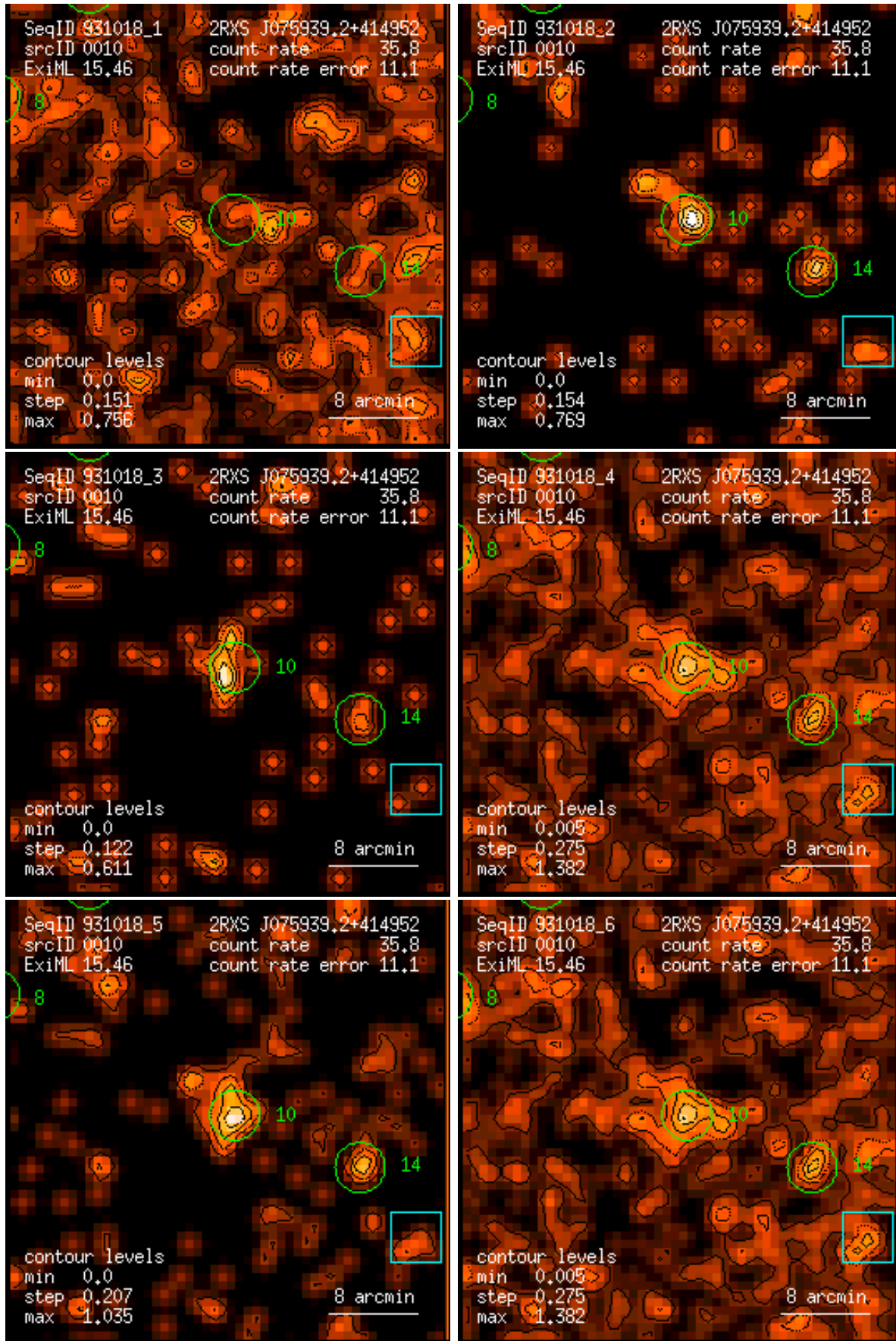
Figure 10: RASS 931018: detection 0010: band rate images, Gaussian filter: (1) PSPC channels 11 – 41, (2) 52 – 90, (3) 91 – 201, (4) 11 – 235, (5) 52 – 201, (6) 11 – 201. Broad band rates in counts/ks. Band rate contour levels in counts/ks/arcmin 2 .
