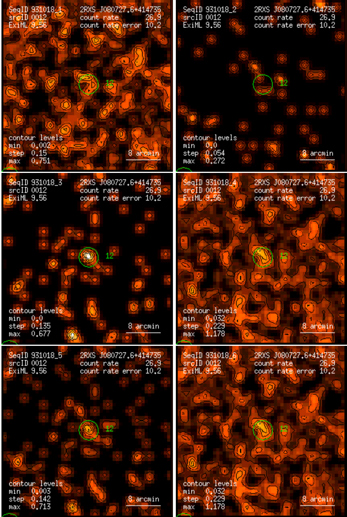
Figure 12: RASS 931018: detection 0012: band rate images, Gaussian filter: (1) PSPC channels 11 – 41, (2) 52 – 90, (3) 91 – 201, (4) 11 – 235, (5) 52 – 201, (6) 11 – 201. Broad band rates in counts/ks. Band rate contour levels in counts/ks/arcmin 2 .
