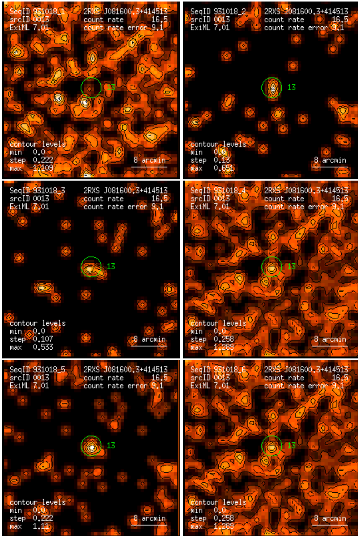
Figure 13: RASS 931018: detection 0013: band rate images, Gaussian filter: (1) PSPC channels 11 – 41, (2) 52 – 90, (3) 91 – 201, (4) 11 – 235, (5) 52 – 201, (6) 11 – 201. Broad band rates in counts/ks. Band rate contour levels in counts/ks/arcmin 2 .
