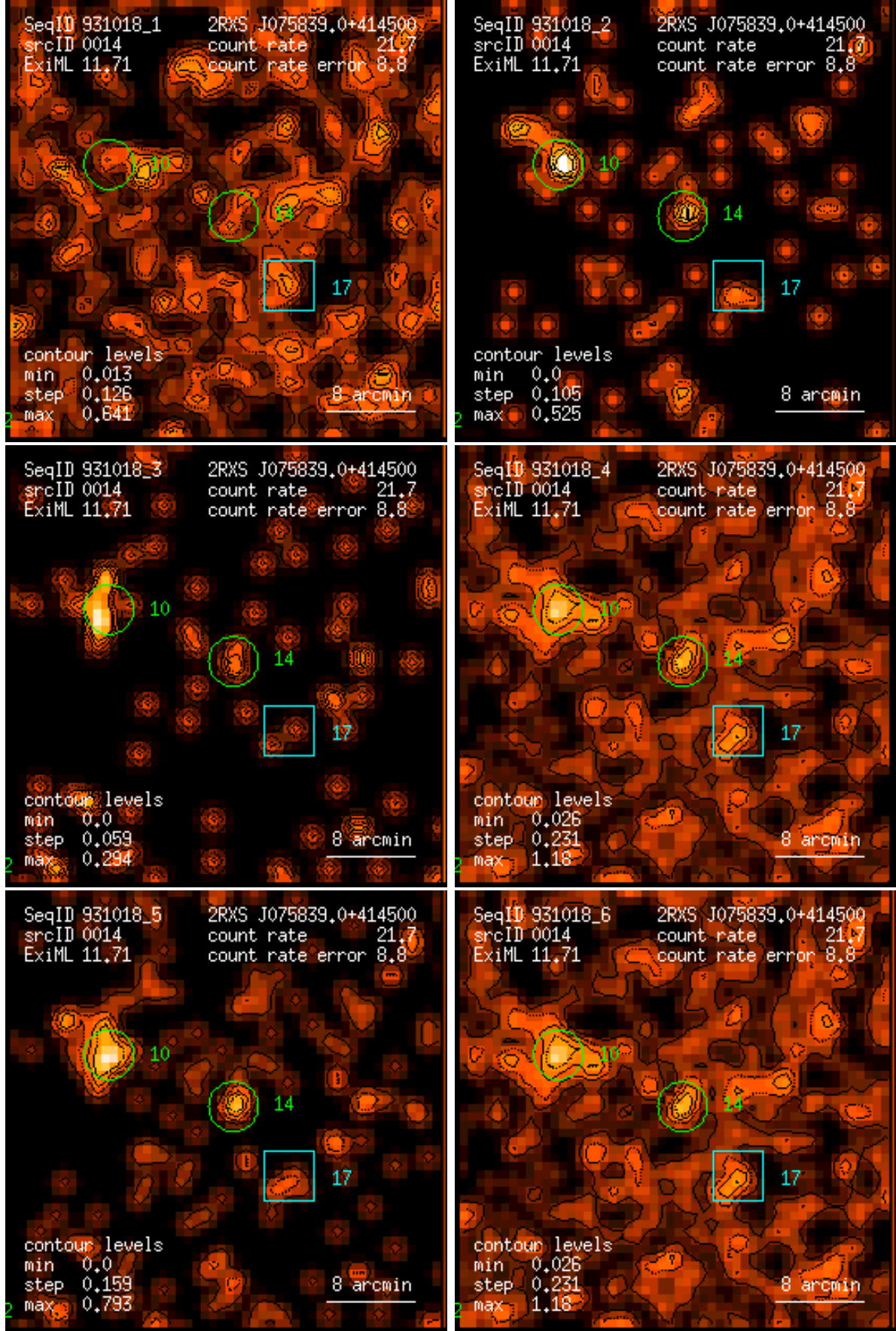
Figure 14: RASS 931018: detection 0014: band rate images, Gaussian filter: (1) PSPC channels 11 – 41, (2) 52 – 90, (3) 91 – 201, (4) 11 – 235, (5) 52 – 201, (6) 11 – 201. Broad band rates in counts/ks. Band rate contour levels in counts/ks/arcmin 2 .
