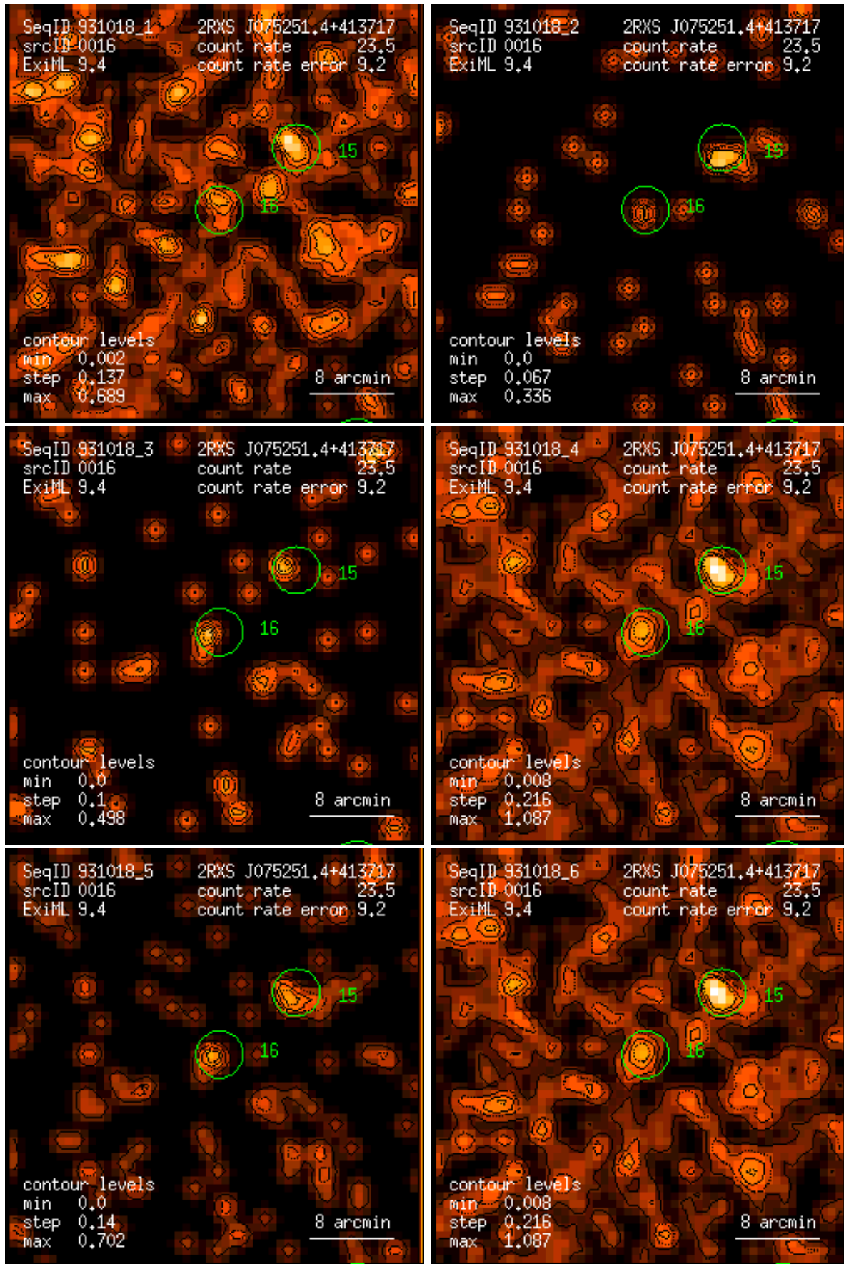
Figure 16: RASS 931018: detection 0016: band rate images, Gaussian filter: (1) PSPC channels 11 – 41, (2) 52 – 90, (3) 91 – 201, (4) 11 – 235, (5) 52 – 201, (6) 11 – 201. Broad band rates in counts/ks. Band rate contour levels in counts/ks/arcmin 2 .
