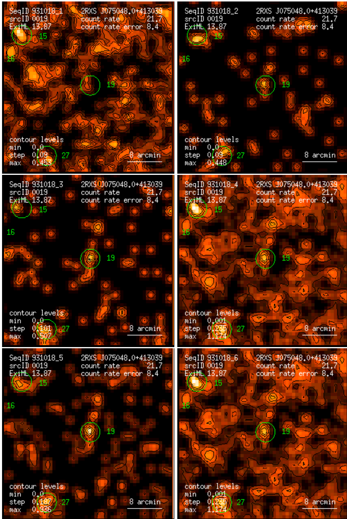
Figure 19: RASS 931018: detection 0019: band rate images, Gaussian filter: (1) PSPC channels 11 – 41, (2) 52 – 90, (3) 91 – 201, (4) 11 – 235, (5) 52 – 201, (6) 11 – 201. Broad band rates in counts/ks. Band rate contour levels in counts/ks/arcmin 2 .
