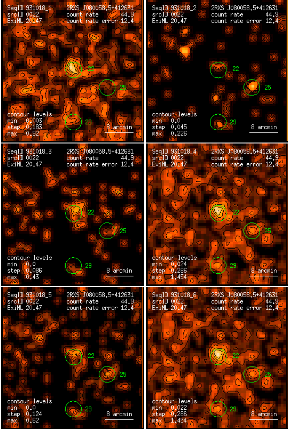
Figure 22: RASS 931018: detection 0022: band rate images, Gaussian filter: (1) PSPC channels 11 – 41, (2) 52 – 90, (3) 91 – 201, (4) 11 – 235, (5) 52 – 201, (6) 11 – 201. Broad band rates in counts/ks. Band rate contour levels in counts/ks/arcmin 2 .
