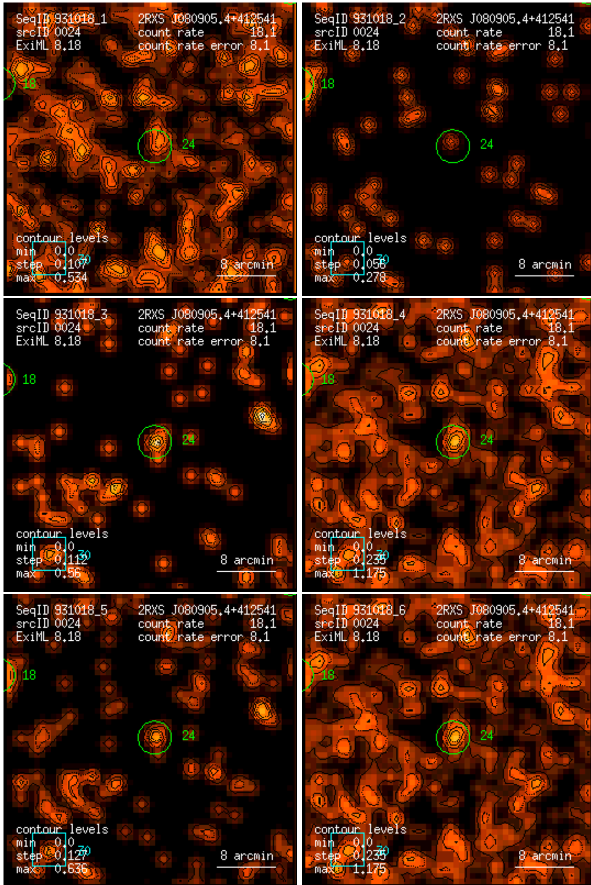
Figure 24: RASS 931018: detection 0024: band rate images, Gaussian filter: (1) PSPC channels 11 – 41, (2) 52 – 90, (3) 91 – 201, (4) 11 – 235, (5) 52 – 201, (6) 11 – 201. Broad band rates in counts/ks. Band rate contour levels in counts/ks/arcmin 2 .
