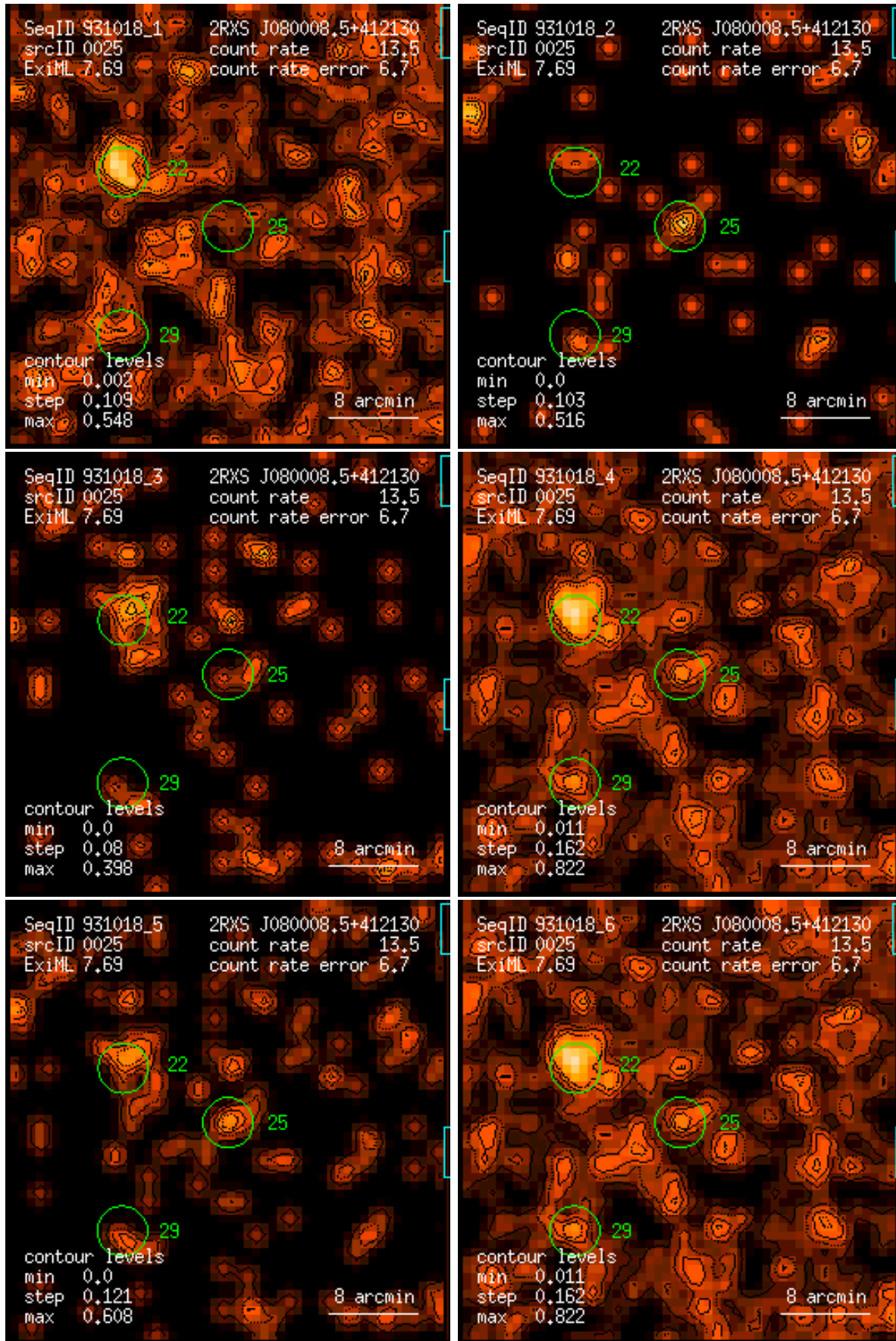
Figure 25: RASS 931018: detection 0025: band rate images, Gaussian filter: (1) PSPC channels 11 – 41, (2) 52 – 90, (3) 91 – 201, (4) 11 – 235, (5) 52 – 201, (6) 11 – 201. Broad band rates in counts/ks. Band rate contour levels in counts/ks/arcmin 2 .
