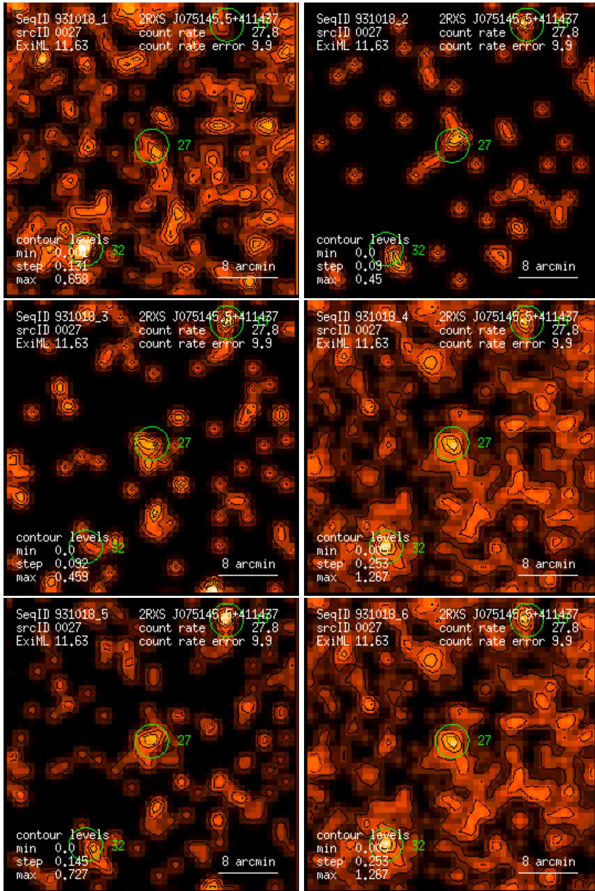
Figure 27: RASS 931018: detection 0027: band rate images, Gaussian filter: (1) PSPC channels 11 – 41, (2) 52 – 90, (3) 91 – 201, (4) 11 – 235, (5) 52 – 201, (6) 11 – 201. Broad band rates in counts/ks. Band rate contour levels in counts/ks/arcmin 2 .
