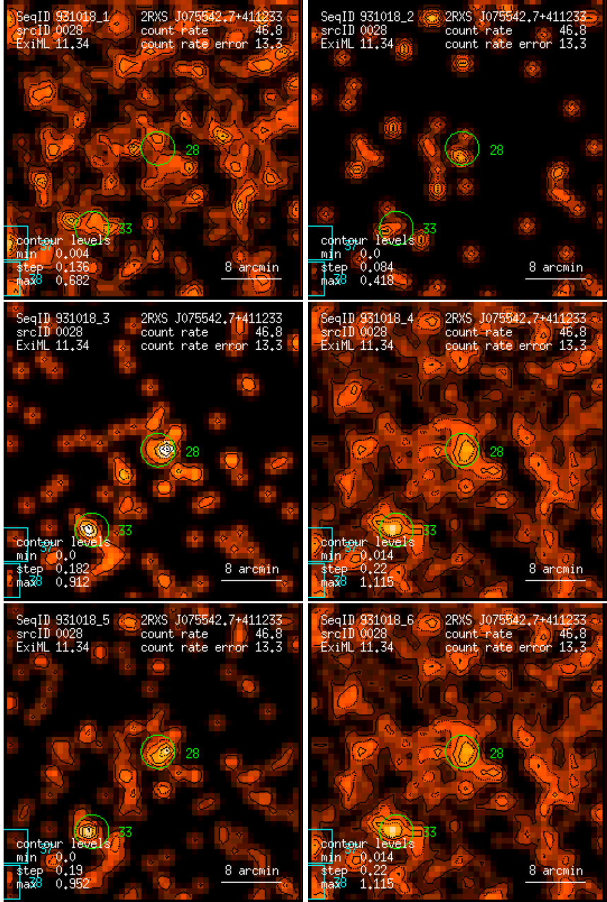
Figure 28: RASS 931018: detection 0028: band rate images, Gaussian filter: (1) PSPC channels 11 – 41, (2) 52 – 90, (3) 91 – 201, (4) 11 – 235, (5) 52 – 201, (6) 11 – 201. Broad band rates in counts/ks. Band rate contour levels in counts/ks/arcmin 2 .
