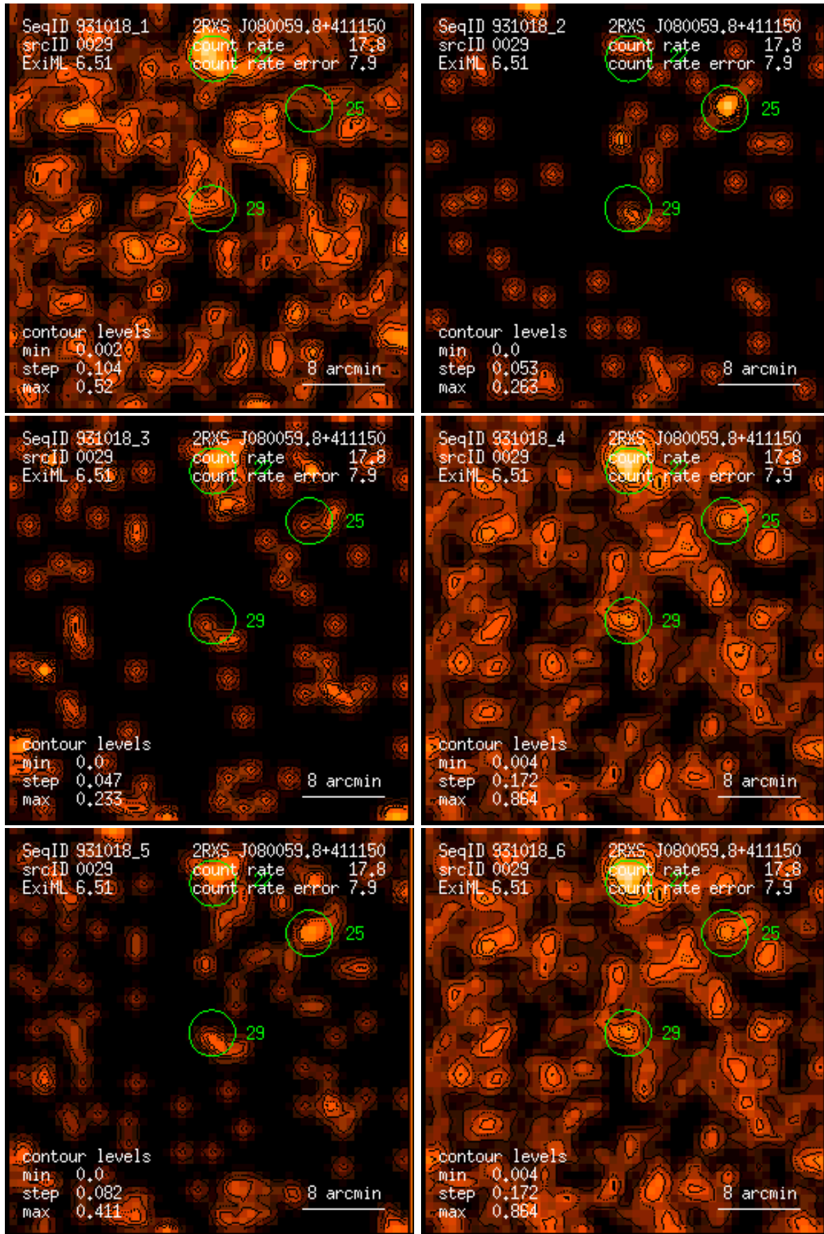
Figure 29: RASS 931018: detection 0029: band rate images, Gaussian filter: (1) PSPC channels 11 – 41, (2) 52 – 90, (3) 91 – 201, (4) 11 – 235, (5) 52 – 201, (6) 11 – 201. Broad band rates in counts/ks. Band rate contour levels in counts/ks/arcmin 2 .
