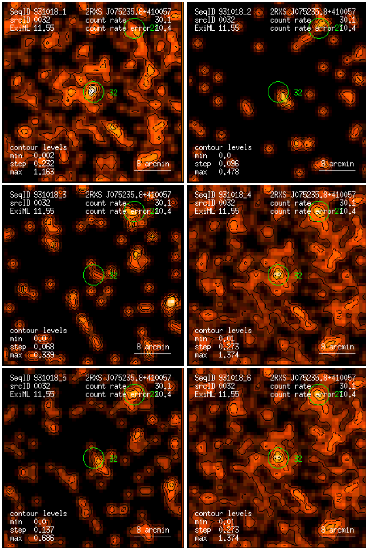
Figure 32: RASS 931018: detection 0032: band rate images, Gaussian filter: (1) PSPC channels 11 – 41, (2) 52 – 90, (3) 91 – 201, (4) 11 – 235, (5) 52 – 201, (6) 11 – 201. Broad band rates in counts/ks. Band rate contour levels in counts/ks/arcmin 2 .
