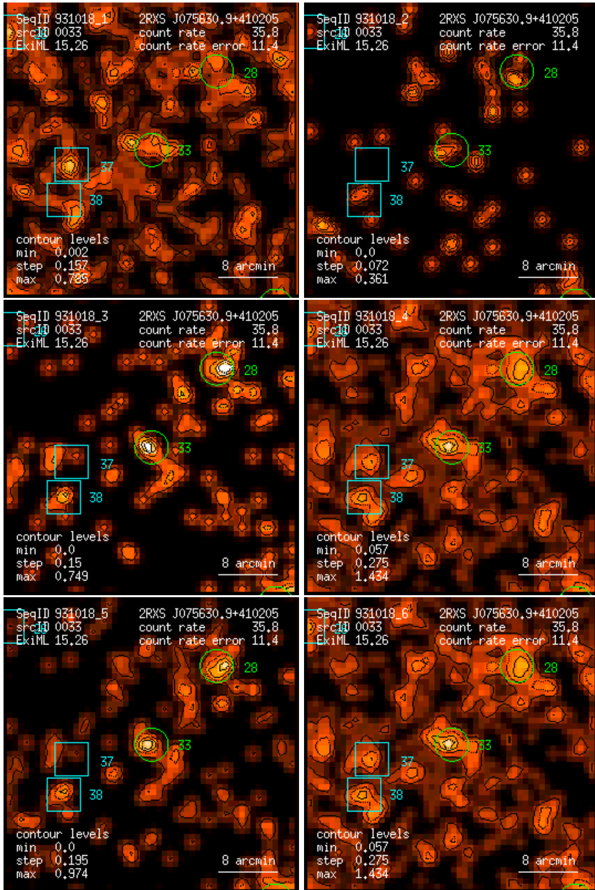
Figure 33: RASS 931018: detection 0033: band rate images, Gaussian filter: (1) PSPC channels 11 – 41, (2) 52 – 90, (3) 91 – 201, (4) 11 – 235, (5) 52 – 201, (6) 11 – 201. Broad band rates in counts/ks. Band rate contour levels in counts/ks/arcmin 2 .
