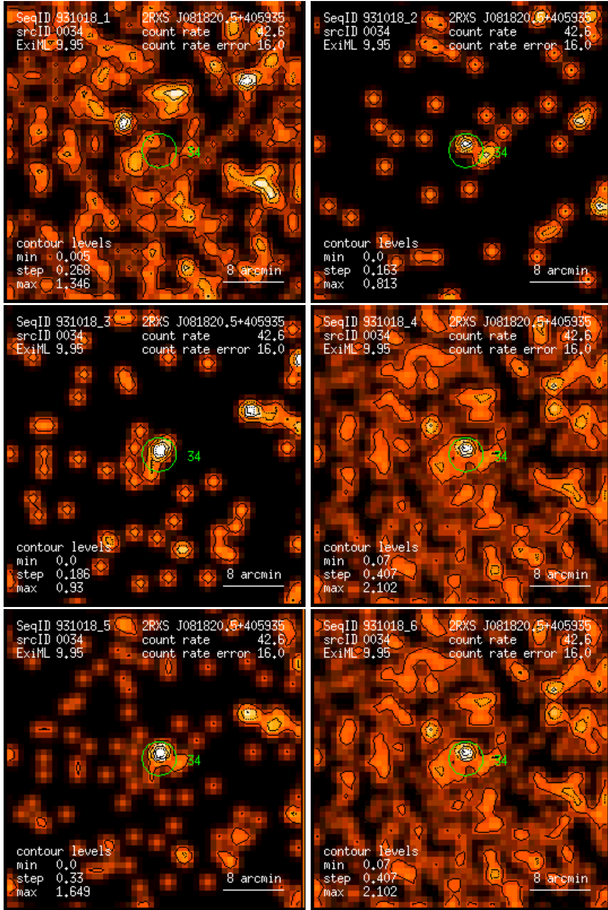
Figure 34: RASS 931018: detection 0034: band rate images, Gaussian filter: (1) PSPC channels 11 – 41, (2) 52 – 90, (3) 91 – 201, (4) 11 – 235, (5) 52 – 201, (6) 11 – 201. Broad band rates in counts/ks. Band rate contour levels in counts/ks/arcmin 2 .
