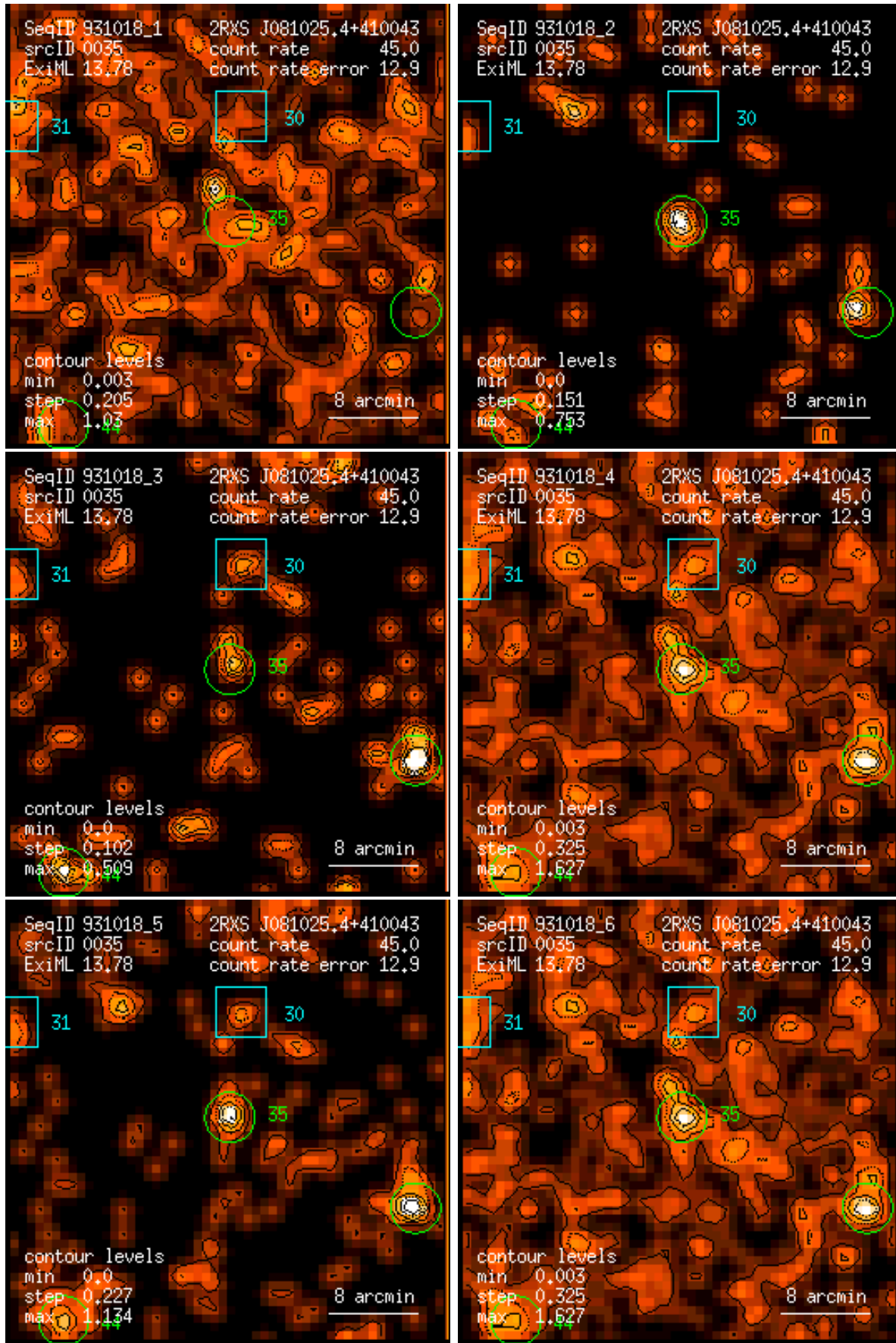
Figure 35: RASS 931018: detection 0035: band rate images, Gaussian filter: (1) PSPC channels 11 – 41, (2) 52 – 90, (3) 91 – 201, (4) 11 – 235, (5) 52 – 201, (6) 11 – 201. Broad band rates in counts/ks. Band rate contour levels in counts/ks/arcmin 2 .
