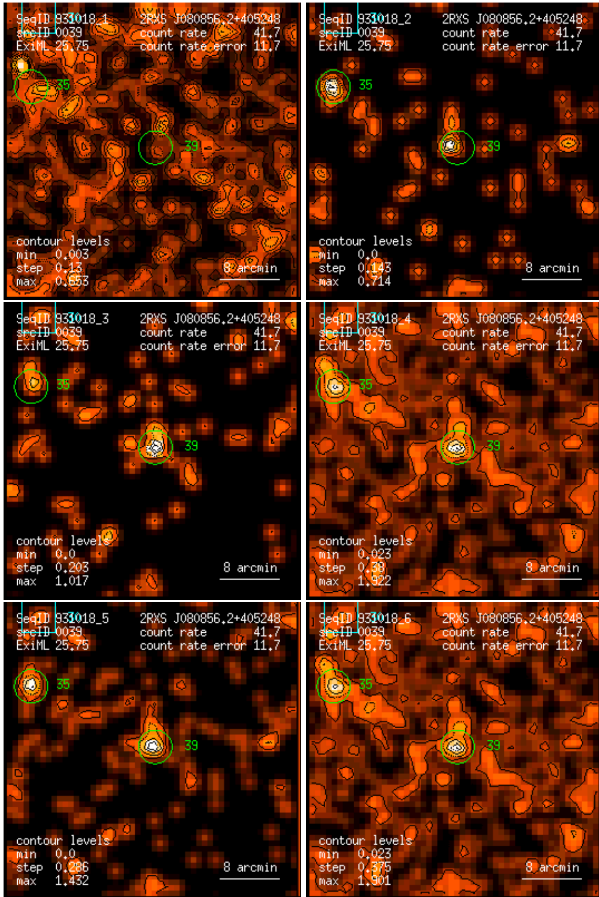
Figure 39: RASS 931018: detection 0039: band rate images, Gaussian filter: (1) PSPC channels 11 – 41, (2) 52 – 90, (3) 91 – 201, (4) 11 – 235, (5) 52 – 201, (6) 11 – 201. Broad band rates in counts/ks. Band rate contour levels in counts/ks/arcmin 2 .
