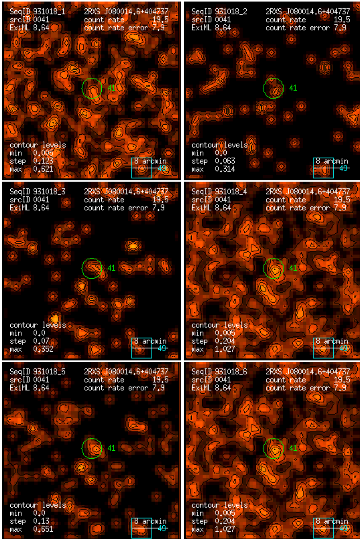
Figure 41: RASS 931018: detection 0041: band rate images, Gaussian filter: (1) PSPC channels 11 – 41, (2) 52 – 90, (3) 91 – 201, (4) 11 – 235, (5) 52 – 201, (6) 11 – 201. Broad band rates in counts/ks. Band rate contour levels in counts/ks/arcmin 2 .
