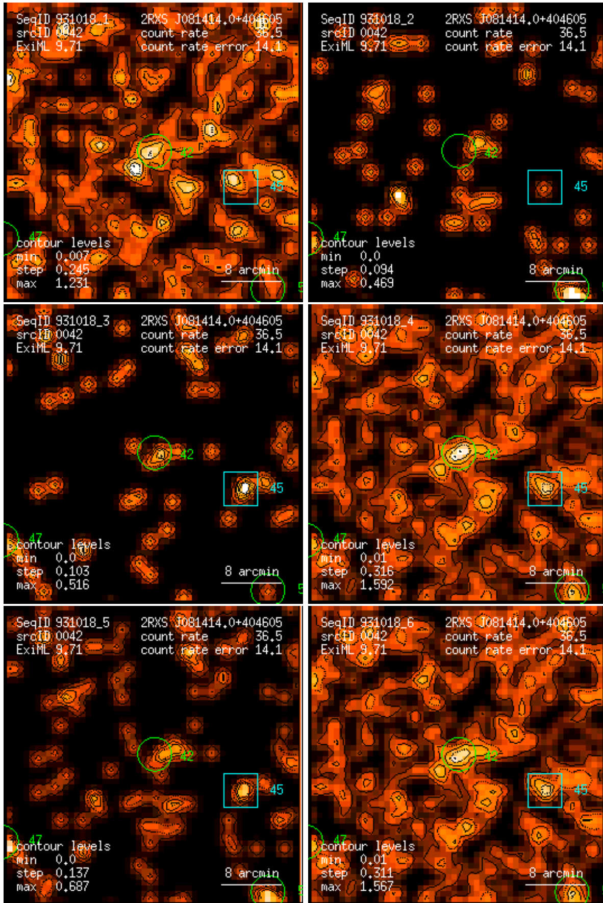
Figure 42: RASS 931018: detection 0042: band rate images, Gaussian filter: (1) PSPC channels 11 – 41, (2) 52 – 90, (3) 91 – 201, (4) 11 – 235, (5) 52 – 201, (6) 11 – 201. Broad band rates in counts/ks. Band rate contour levels in counts/ks/arcmin 2 .
