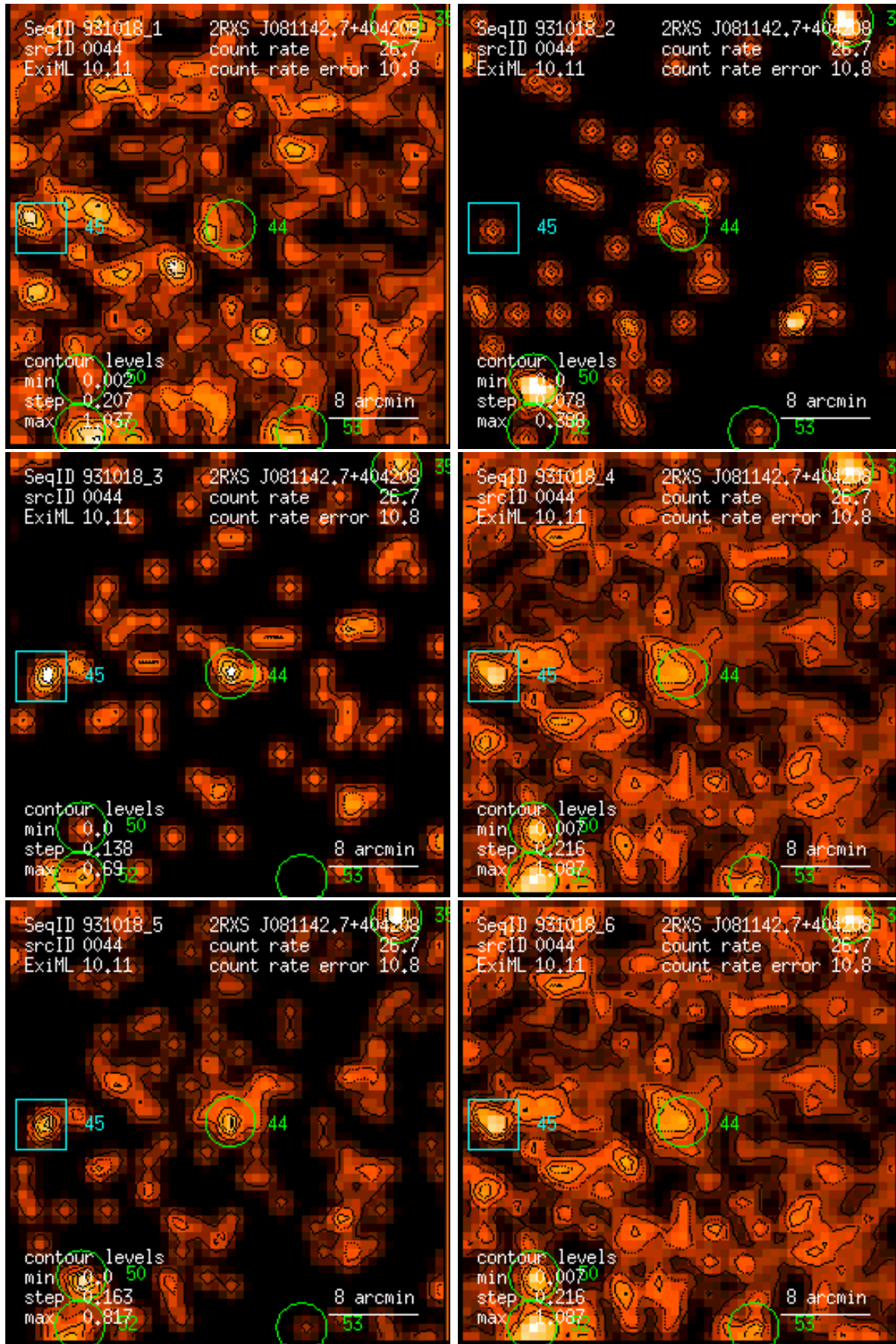
Figure 44: RASS 931018: detection 0044: band rate images, Gaussian filter: (1) PSPC channels 11 – 41, (2) 52 – 90, (3) 91 – 201, (4) 11 – 235, (5) 52 – 201, (6) 11 – 201. Broad band rates in counts/ks. Band rate contour levels in counts/ks/arcmin 2 .
