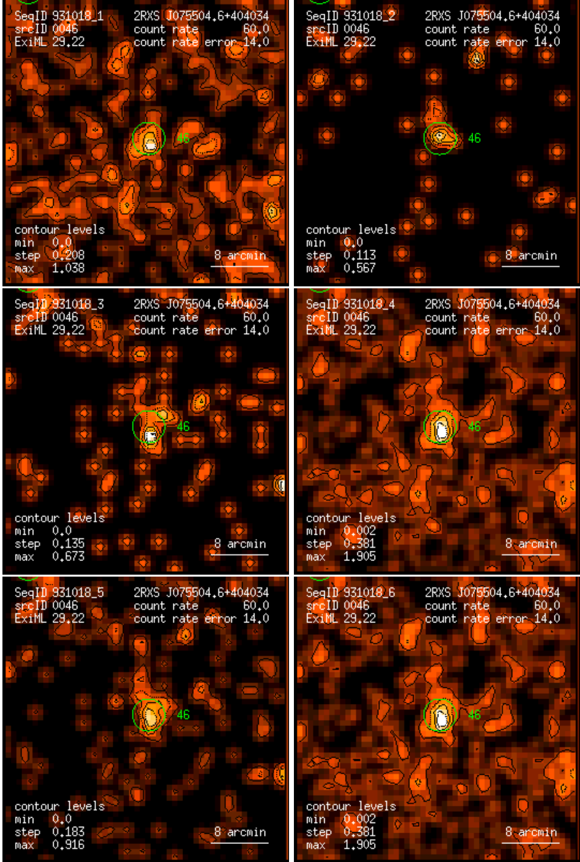
Figure 46: RASS 931018: detection 0046: band rate images, Gaussian filter: (1) PSPC channels 11 – 41, (2) 52 – 90, (3) 91 – 201, (4) 11 – 235, (5) 52 – 201, (6) 11 – 201. Broad band rates in counts/ks. Band rate contour levels in counts/ks/arcmin 2 .
