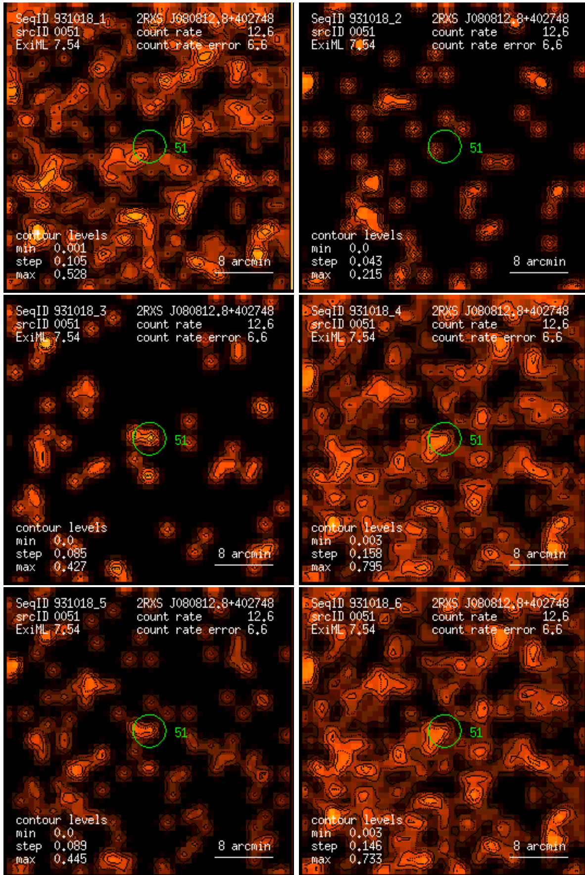
Figure 51: RASS 931018: detection 0051: band rate images, Gaussian filter: (1) PSPC channels 11 – 41, (2) 52 – 90, (3) 91 – 201, (4) 11 – 235, (5) 52 – 201, (6) 11 – 201. Broad band rates in counts/ks. Band rate contour levels in counts/ks/arcmin 2 .
