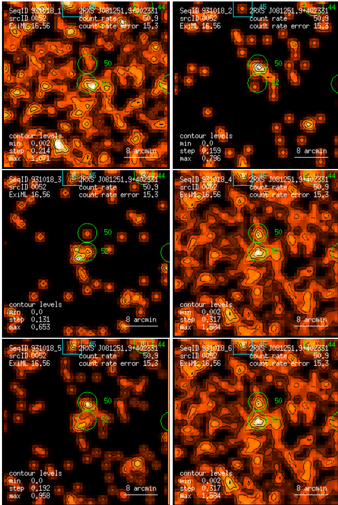
Figure 52: RASS 931018: detection 0052: band rate images, Gaussian filter: (1) PSPC channels 11 – 41, (2) 52 – 90, (3) 91 – 201, (4) 11 – 235, (5) 52 – 201, (6) 11 – 201. Broad band rates in counts/ks. Band rate contour levels in counts/ks/arcmin 2 .
