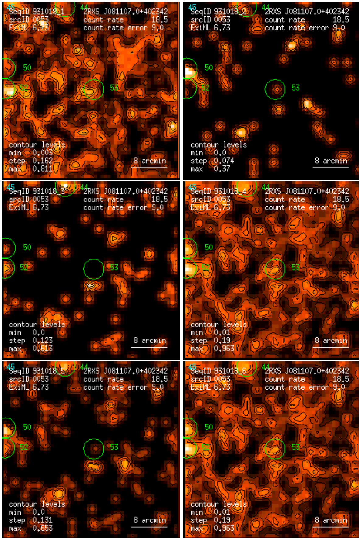
Figure 53: RASS 931018: detection 0053: band rate images, Gaussian filter: (1) PSPC channels 11 – 41, (2) 52 – 90, (3) 91 – 201, (4) 11 – 235, (5) 52 – 201, (6) 11 – 201. Broad band rates in counts/ks. Band rate contour levels in counts/ks/arcmin 2 .
