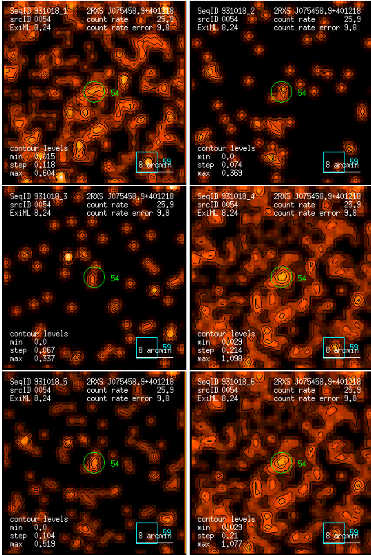
Figure 54: RASS 931018: detection 0054: band rate images, Gaussian filter: (1) PSPC channels 11 – 41, (2) 52 – 90, (3) 91 – 201, (4) 11 – 235, (5) 52 – 201, (6) 11 – 201. Broad band rates in counts/ks. Band rate contour levels in counts/ks/arcmin 2 .
