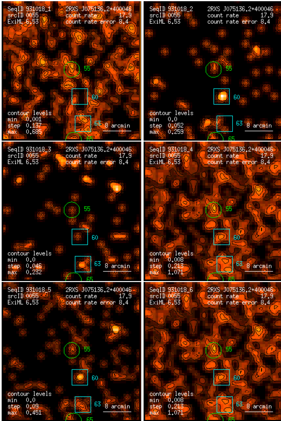
Figure 55: RASS 931018: detection 0055: band rate images, Gaussian filter: (1) PSPC channels 11 – 41, (2) 52 – 90, (3) 91 – 201, (4) 11 – 235, (5) 52 – 201, (6) 11 – 201. Broad band rates in counts/ks. Band rate contour levels in counts/ks/arcmin 2 .
