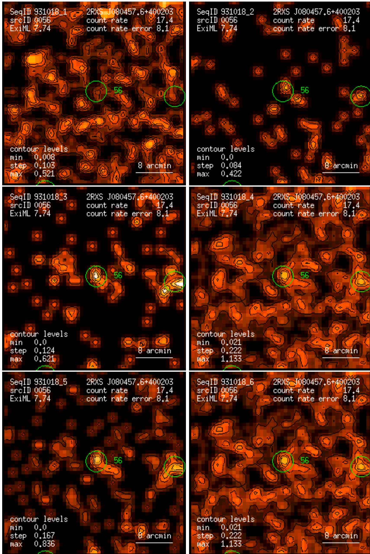
Figure 56: RASS 931018: detection 0056: band rate images, Gaussian filter: (1) PSPC channels 11 – 41, (2) 52 – 90, (3) 91 – 201, (4) 11 – 235, (5) 52 – 201, (6) 11 – 201. Broad band rates in counts/ks. Band rate contour levels in counts/ks/arcmin 2 .
