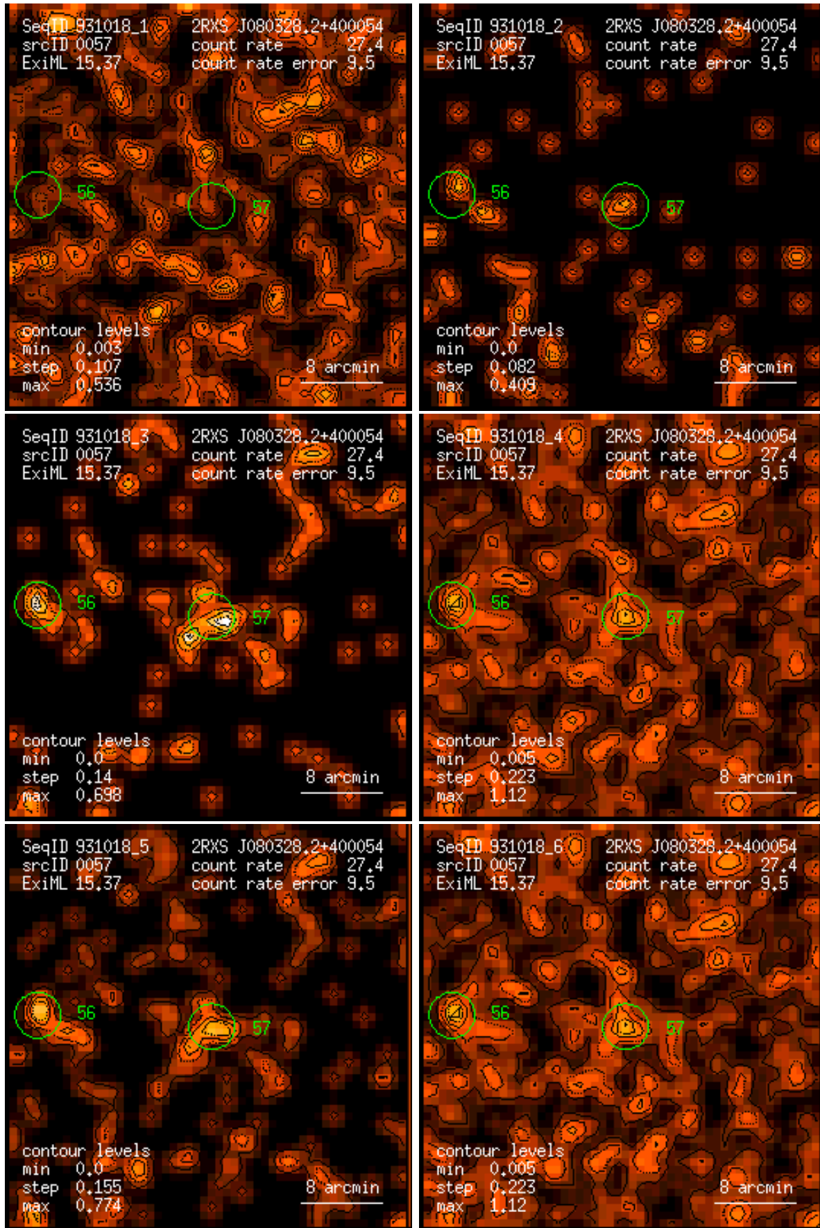
Figure 57: RASS 931018: detection 0057: band rate images, Gaussian filter: (1) PSPC channels 11 – 41, (2) 52 – 90, (3) 91 – 201, (4) 11 – 235, (5) 52 – 201, (6) 11 – 201. Broad band rates in counts/ks. Band rate contour levels in counts/ks/arcmin 2 .
