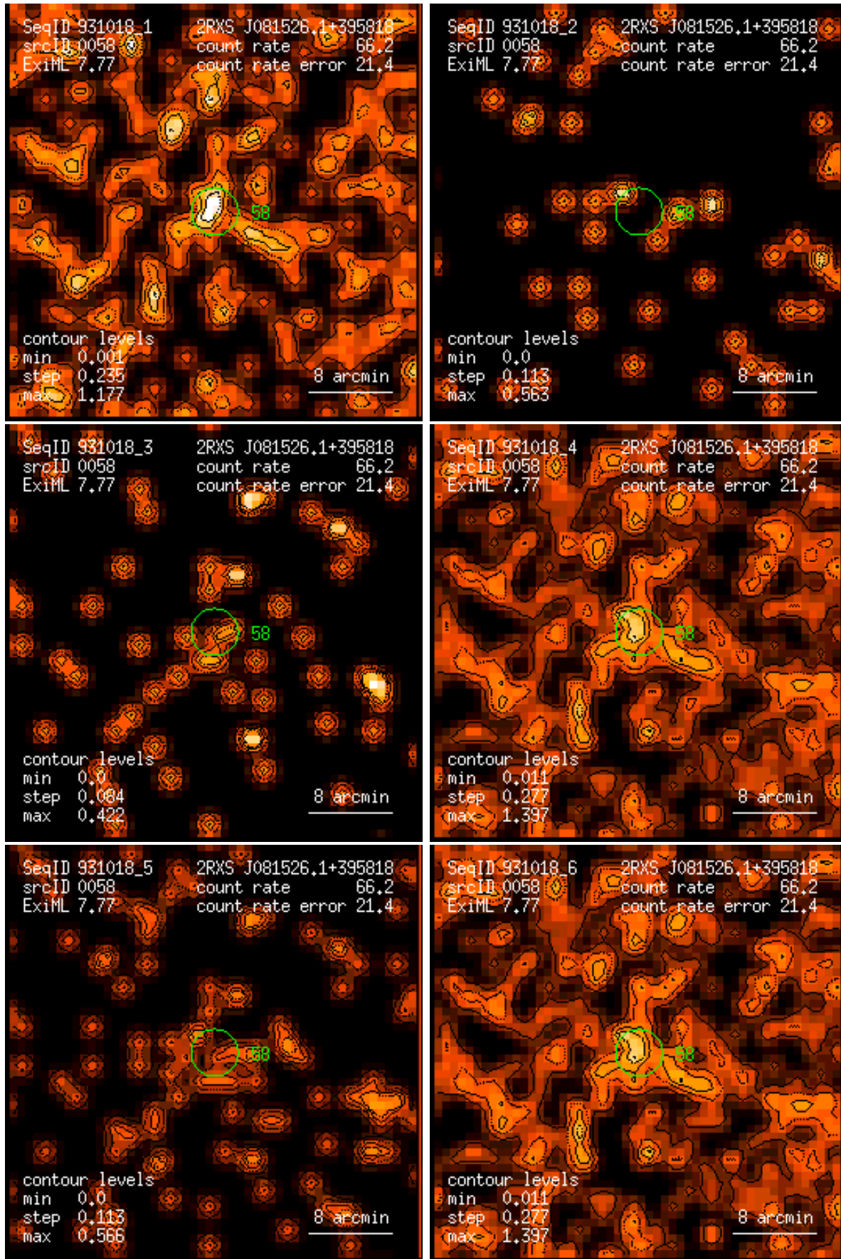
Figure 58: RASS 931018: detection 0058: band rate images, Gaussian filter: (1) PSPC channels 11 – 41, (2) 52 – 90, (3) 91 – 201, (4) 11 – 235, (5) 52 – 201, (6) 11 – 201. Broad band rates in counts/ks. Band rate contour levels in counts/ks/arcmin 2 .
