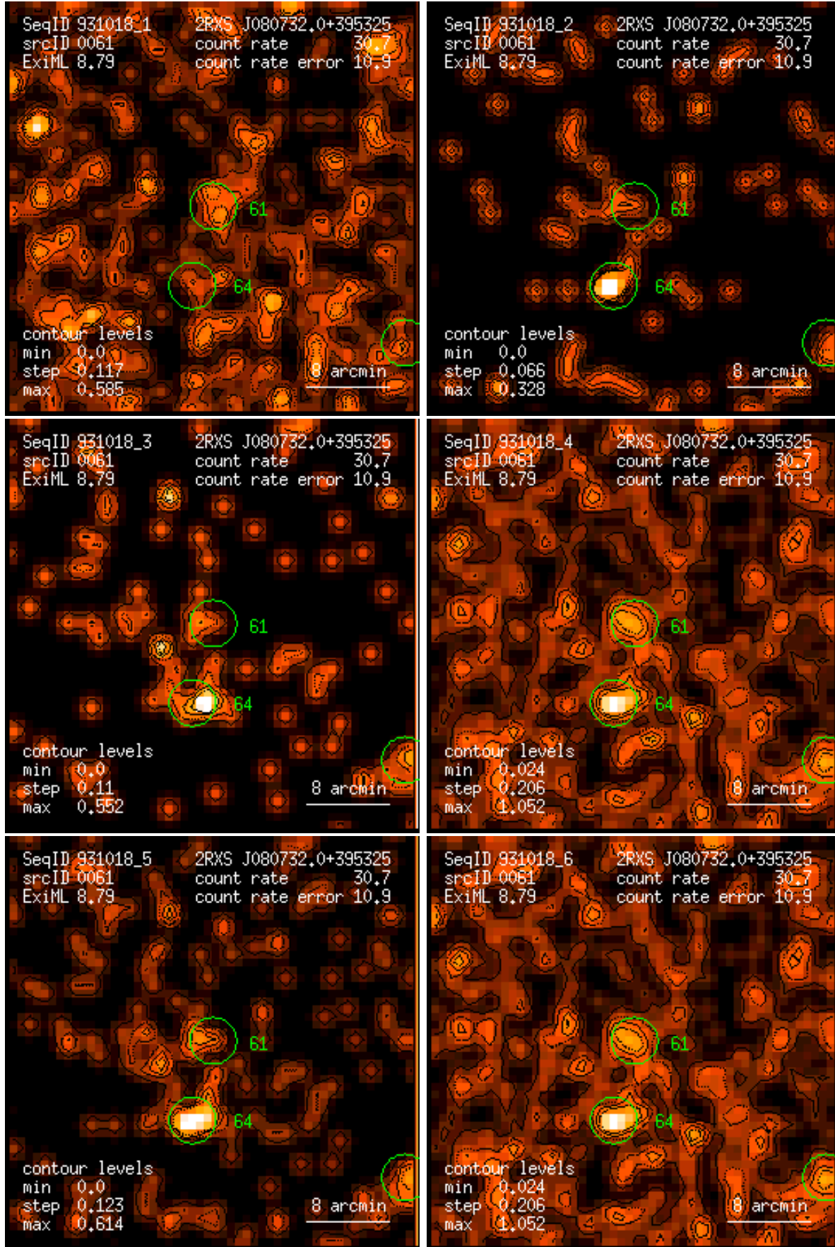
Figure 61: RASS 931018: detection 0061: band rate images, Gaussian filter: (1) PSPC channels 11 – 41, (2) 52 – 90, (3) 91 – 201, (4) 11 – 235, (5) 52 – 201, (6) 11 – 201. Broad band rates in counts/ks. Band rate contour levels in counts/ks/arcmin 2 .
