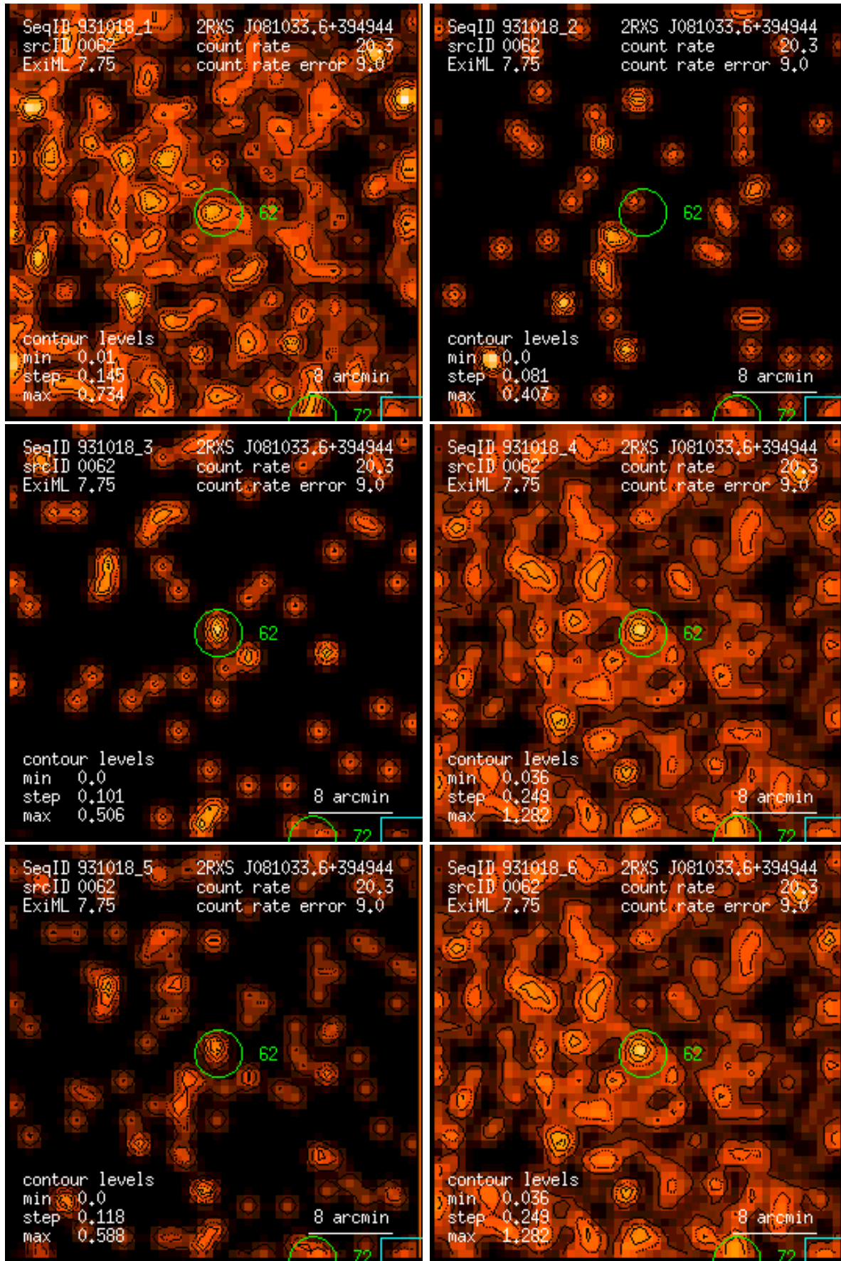
Figure 62: RASS 931018: detection 0062: band rate images, Gaussian filter: (1) PSPC channels 11 – 41, (2) 52 – 90, (3) 91 – 201, (4) 11 – 235, (5) 52 – 201, (6) 11 – 201. Broad band rates in counts/ks. Band rate contour levels in counts/ks/arcmin 2 .
